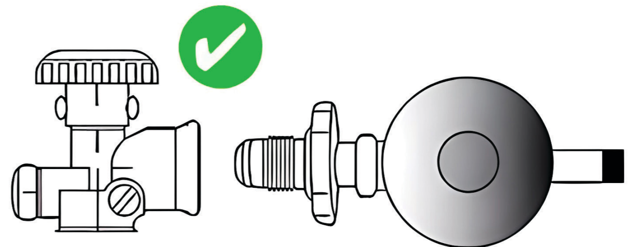
POL valve + POL regulator connection
