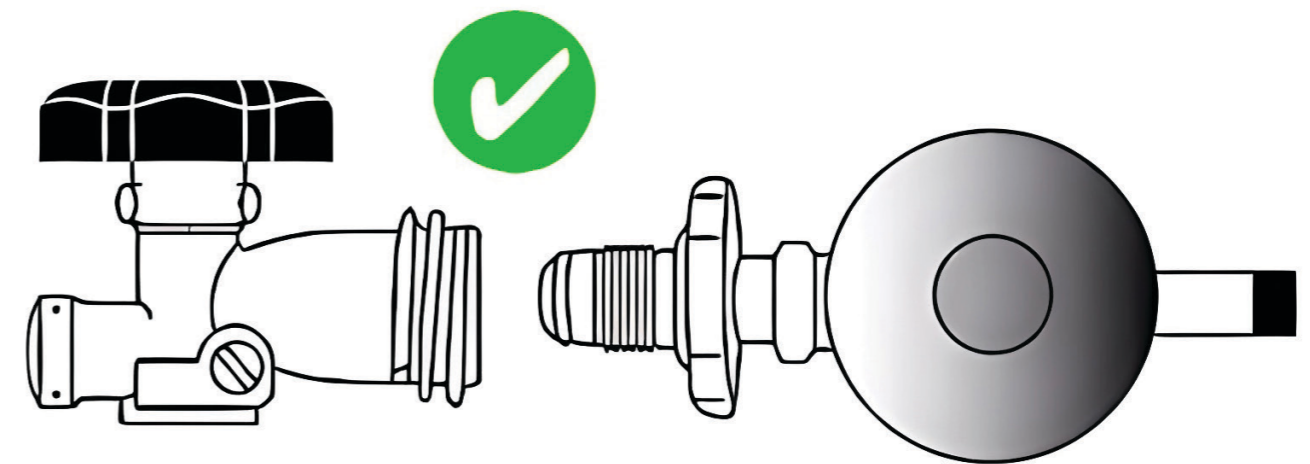
LCC27 valve + POL regulator connection
