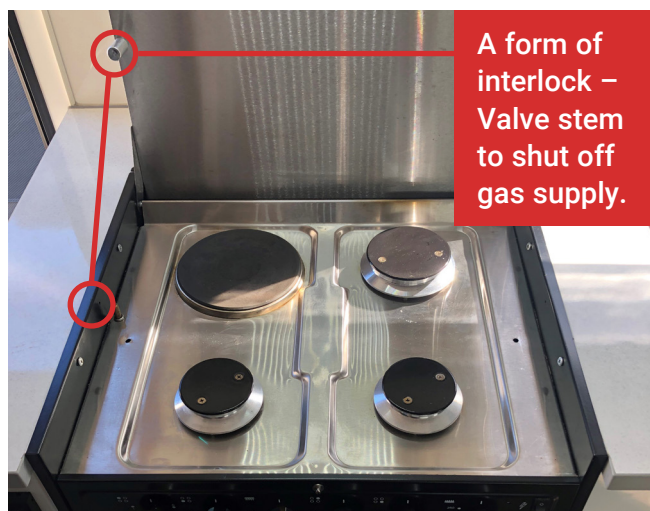
Figure 1 – A typical acceptable 'form of interlock'.
