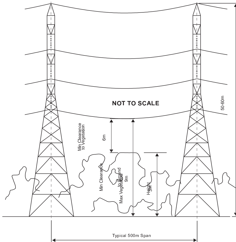
Figure 15: Example of a typical 330kV Transmission line and the associated Vegetation Clearing Profile
