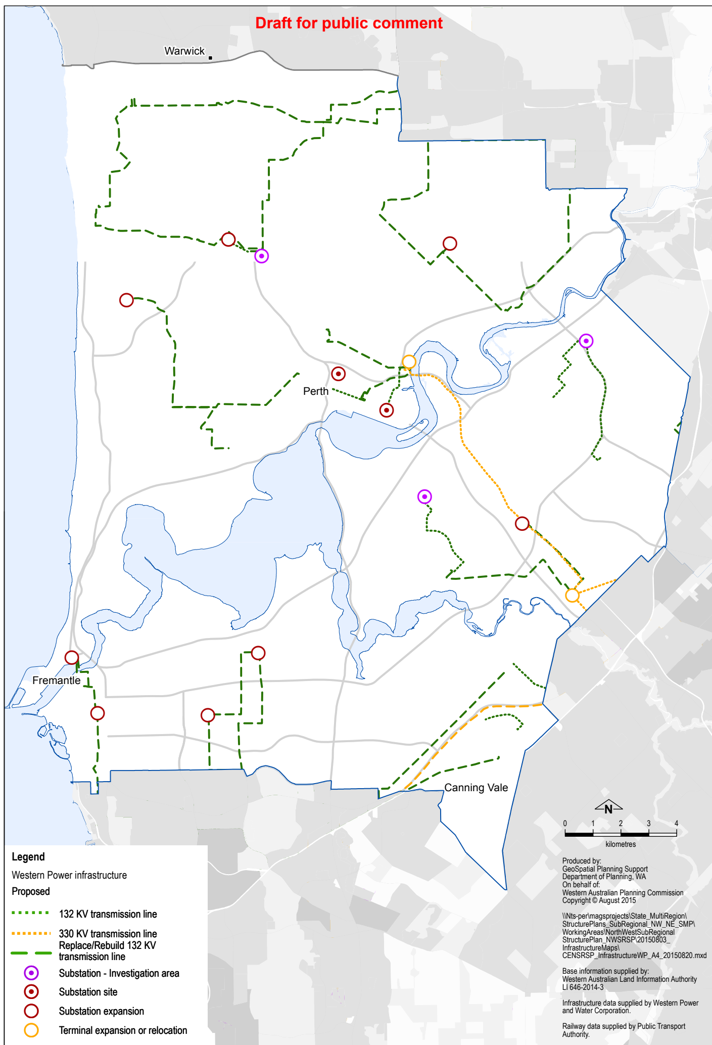
Figure 17: Proposed infrastructure - Western Power – Central sub-region
