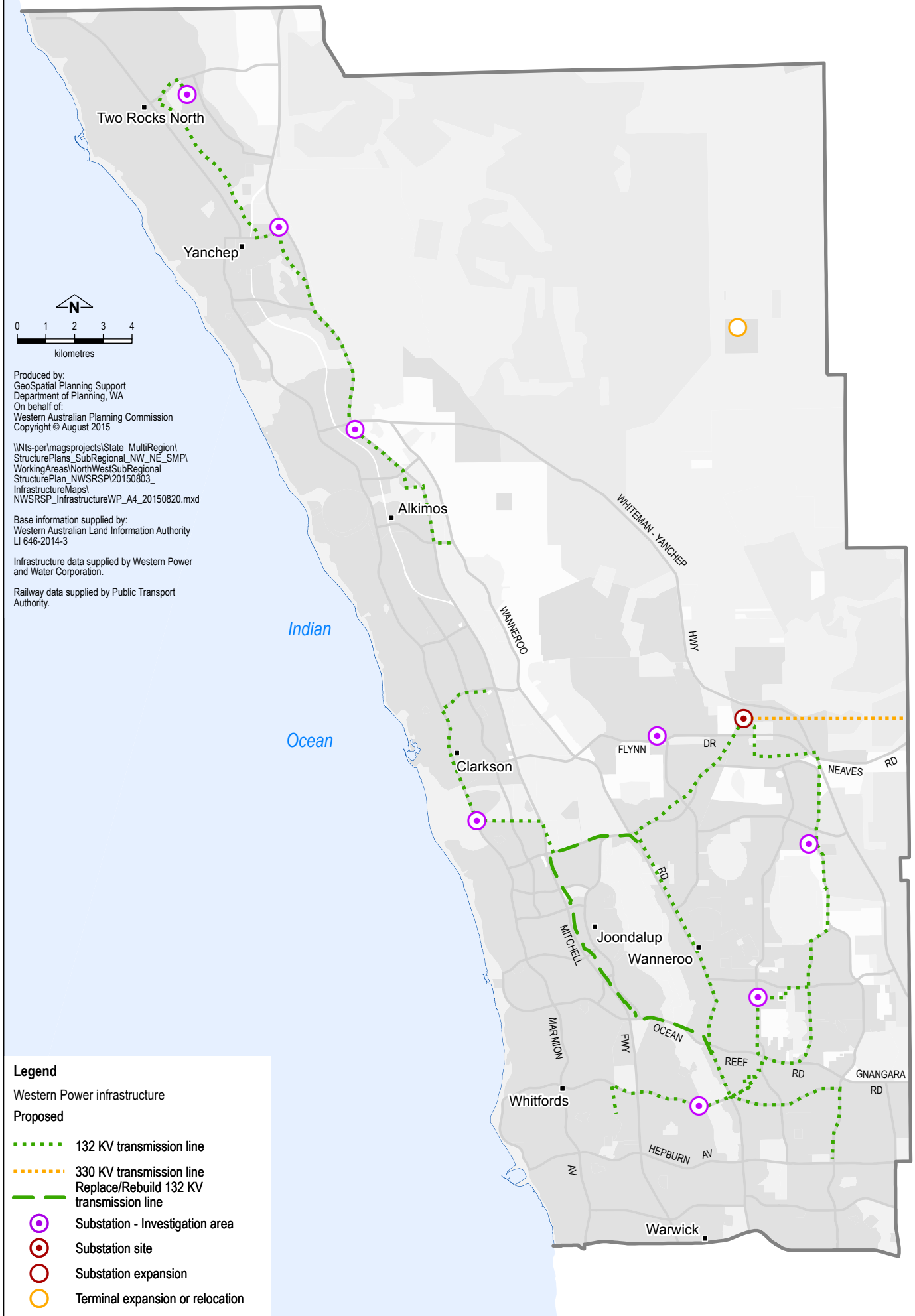
Figure 19: Proposed infrastructure - Western Power – North-West sub-region
