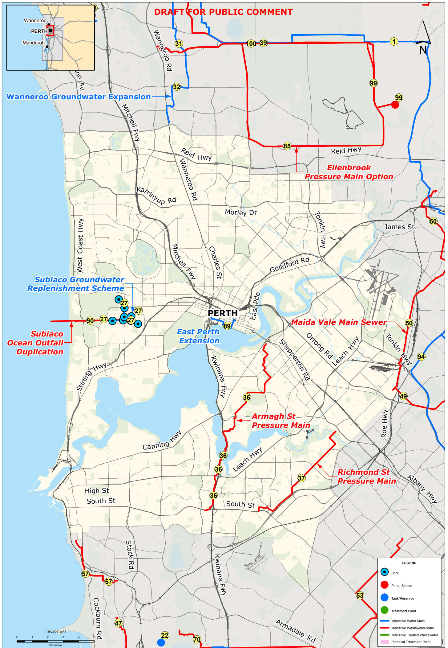
Figure 21: Proposed water and wastewater infrastructure – Central Metropolitan
