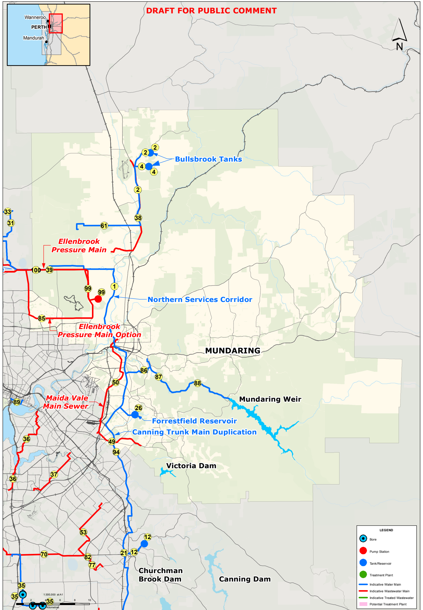
Figure 23: Proposed water and wastewater infrastructure – North-East Metropolitan
