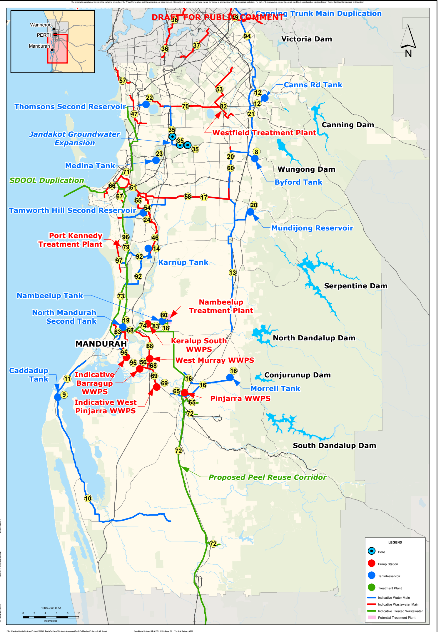
Figure 24: Proposed water and wastewater infrastructure – South Metropolitan and Peel
