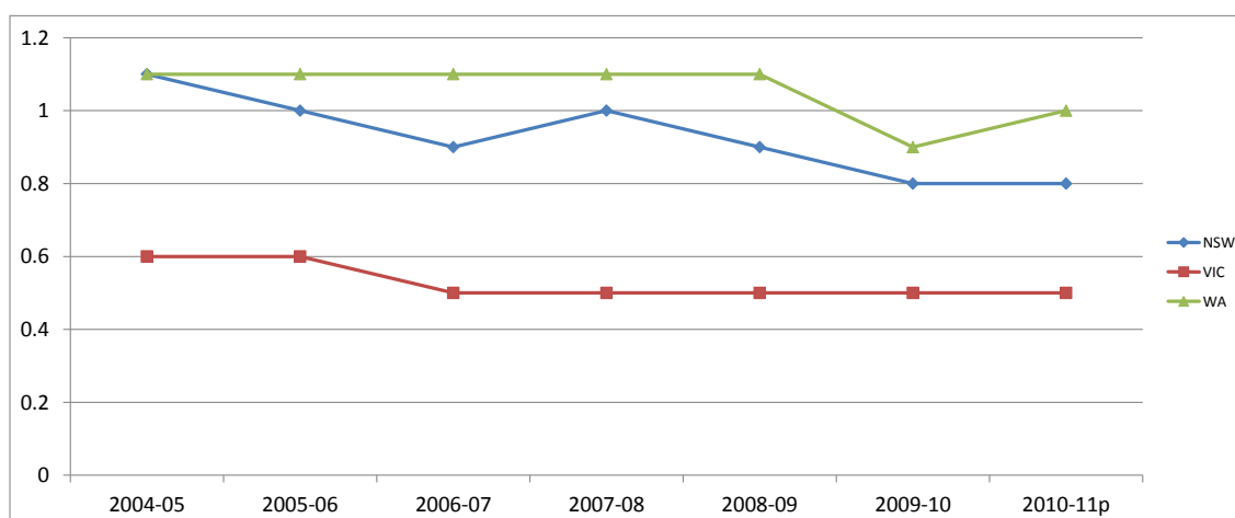
Figure 4: Incidence rate (claims per 1000 employees) of falls from a height in all industries by selected jurisdictions, 2004-05 to 2010-11
