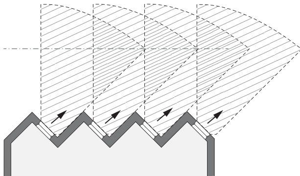
Figure G4.12a Window placement to avoid direct overlooking
