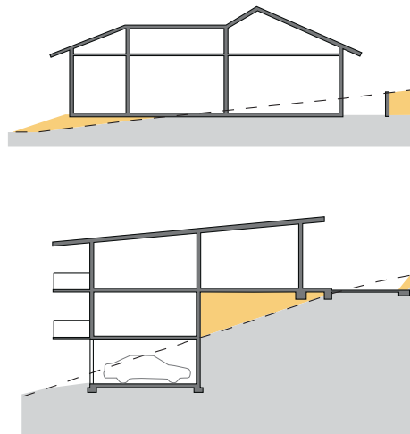
Figure G4.2a Building height for sloping sites
