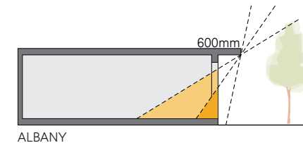
Figure G3.2c Regional variation of eave depths to achieve solar access and shading
