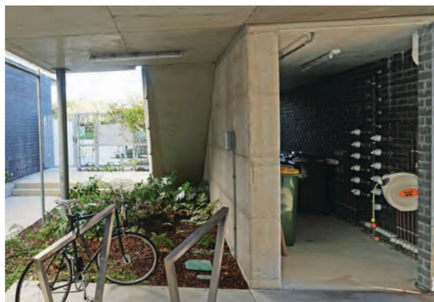
Photo G3.6a and b This bin storage area is conveniently located, neatly integrated into the service area and screened from view
