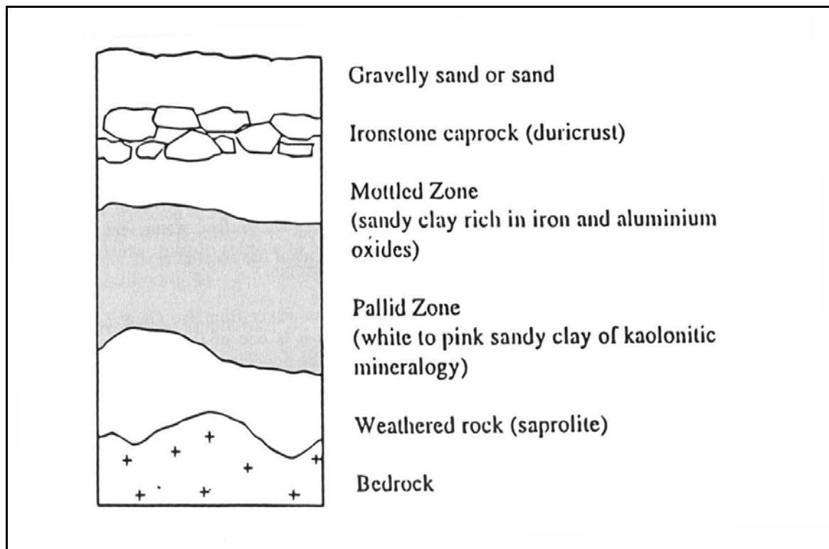
Figure 8: Soil Profile
