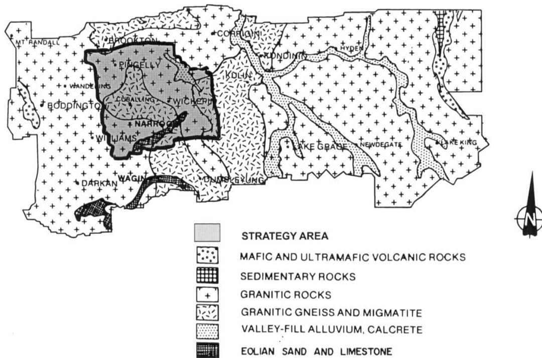
Figure 6: Geology
