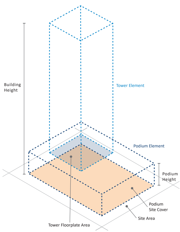
Figure 2: Building Envelope
