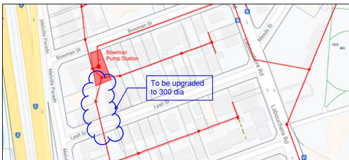
Figure 6 Bowman WWPS gravity sewer upgrade
