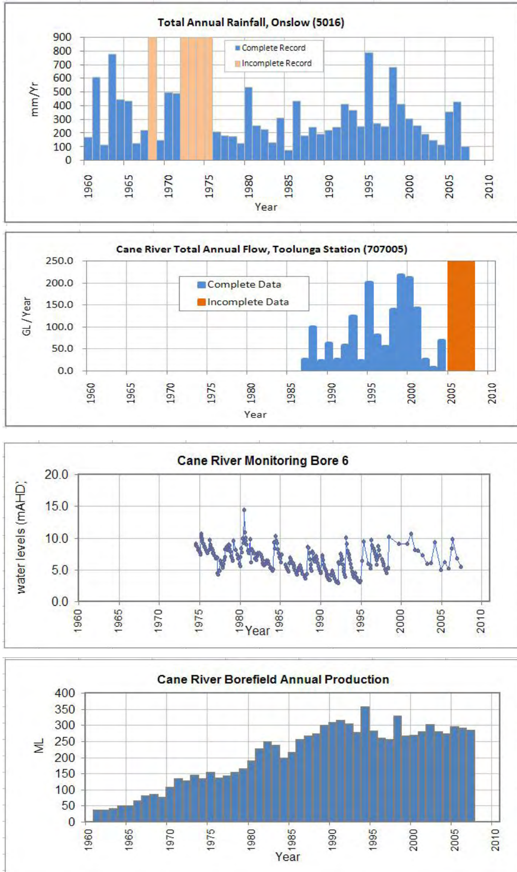
Figure 46: Cane River hydrographs and borefield production
