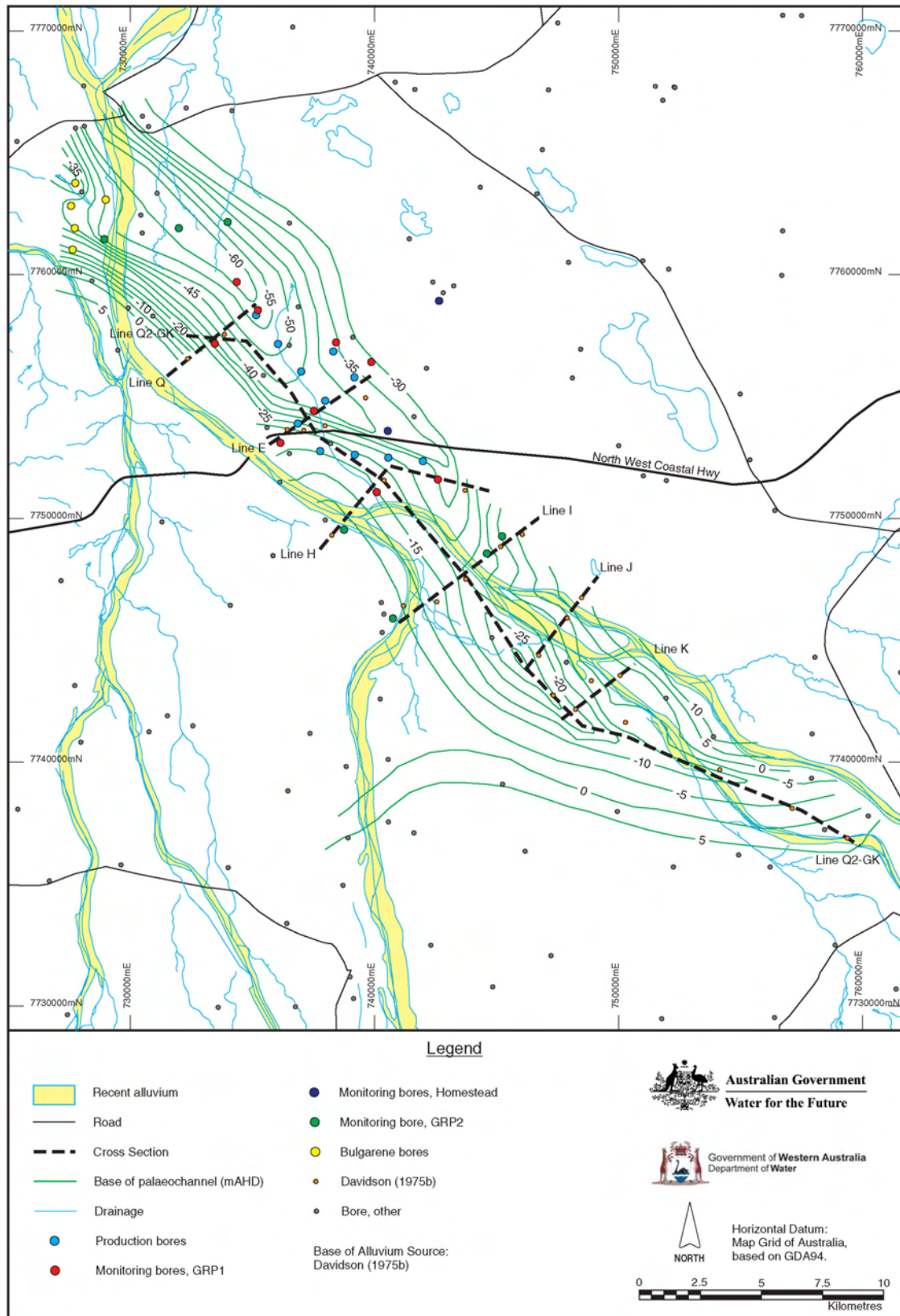
Figure 29: De Grey River base of alluvium
