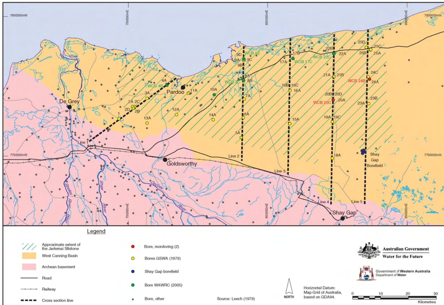
Figure 33: West Canning Basin location
