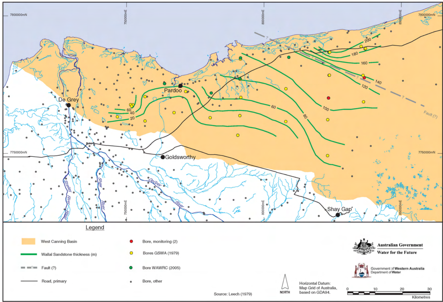
Figure 35: West Canning Basin Wallal Sandstone thickness
