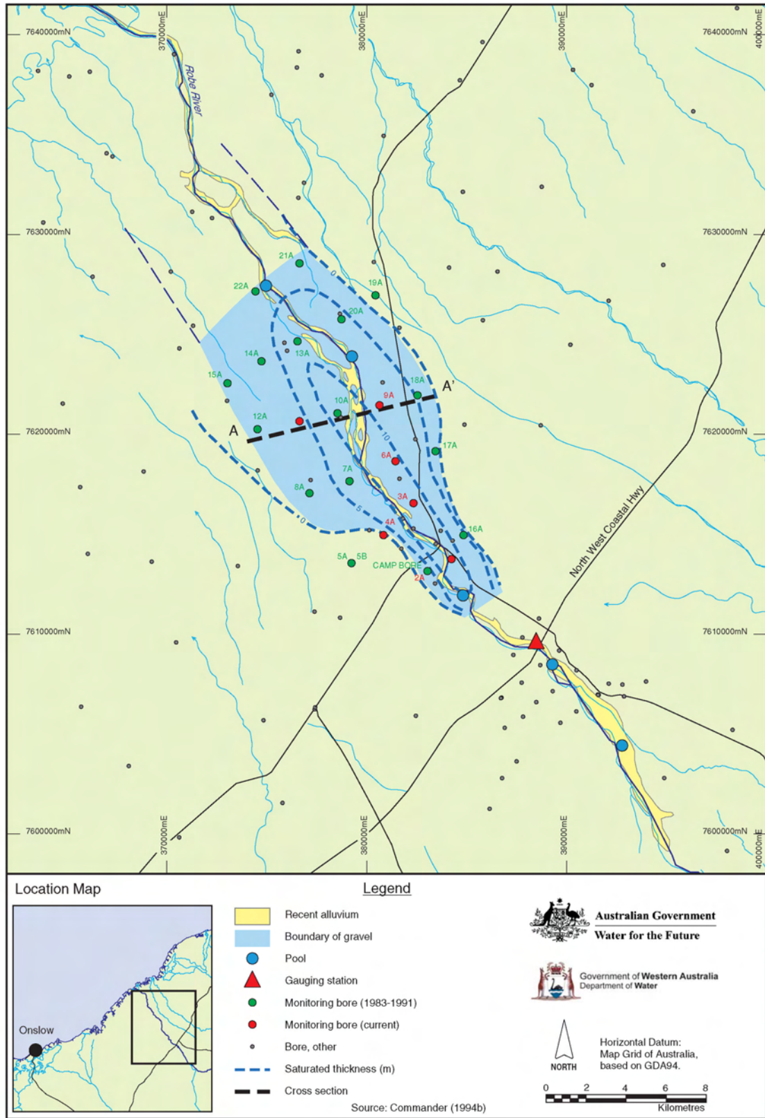
Figure 47: Lower Robe River bores and saturated aquifer thickness
