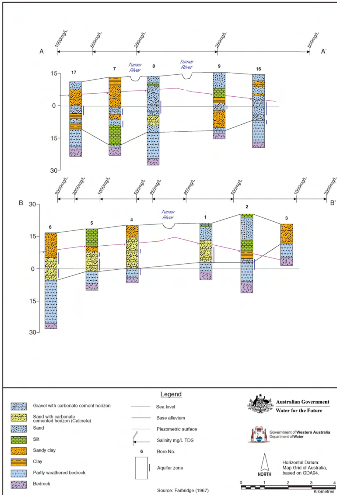
Figure 42: Turner River Area cross sections A and B
