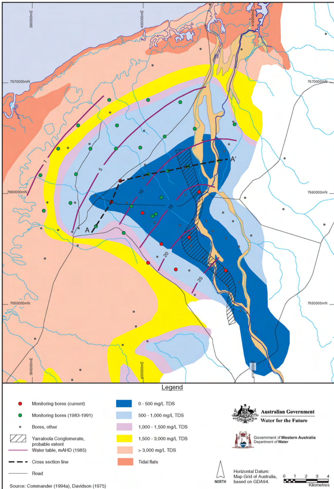
Figure 18: Lower Fortescue River groundwater levels and salinity
