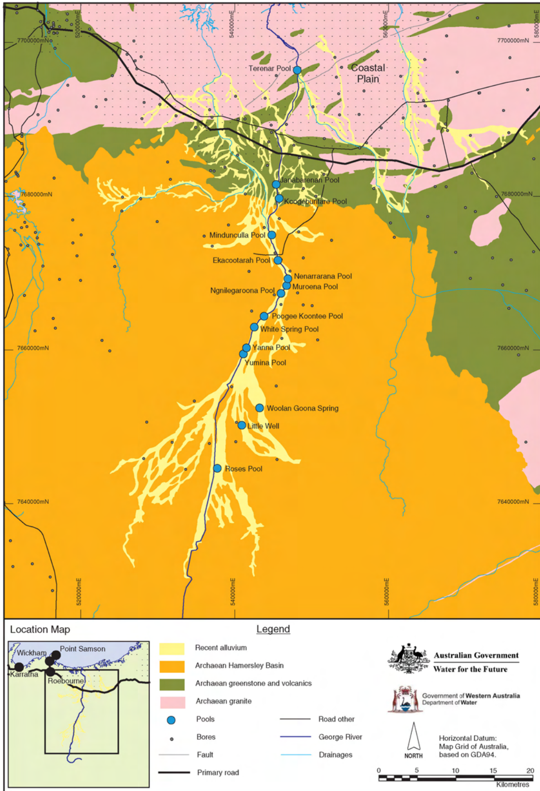
Figure 22: George River Area
