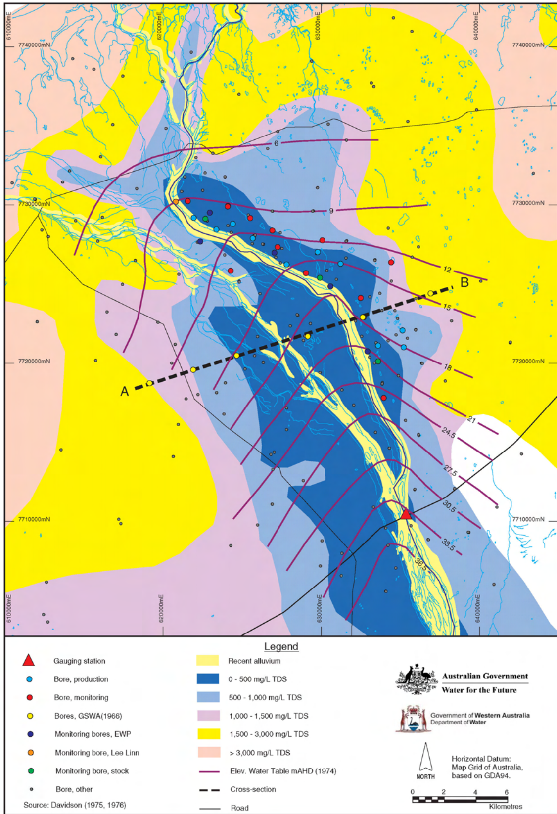
Figure 26: Yule River water table and salinity
