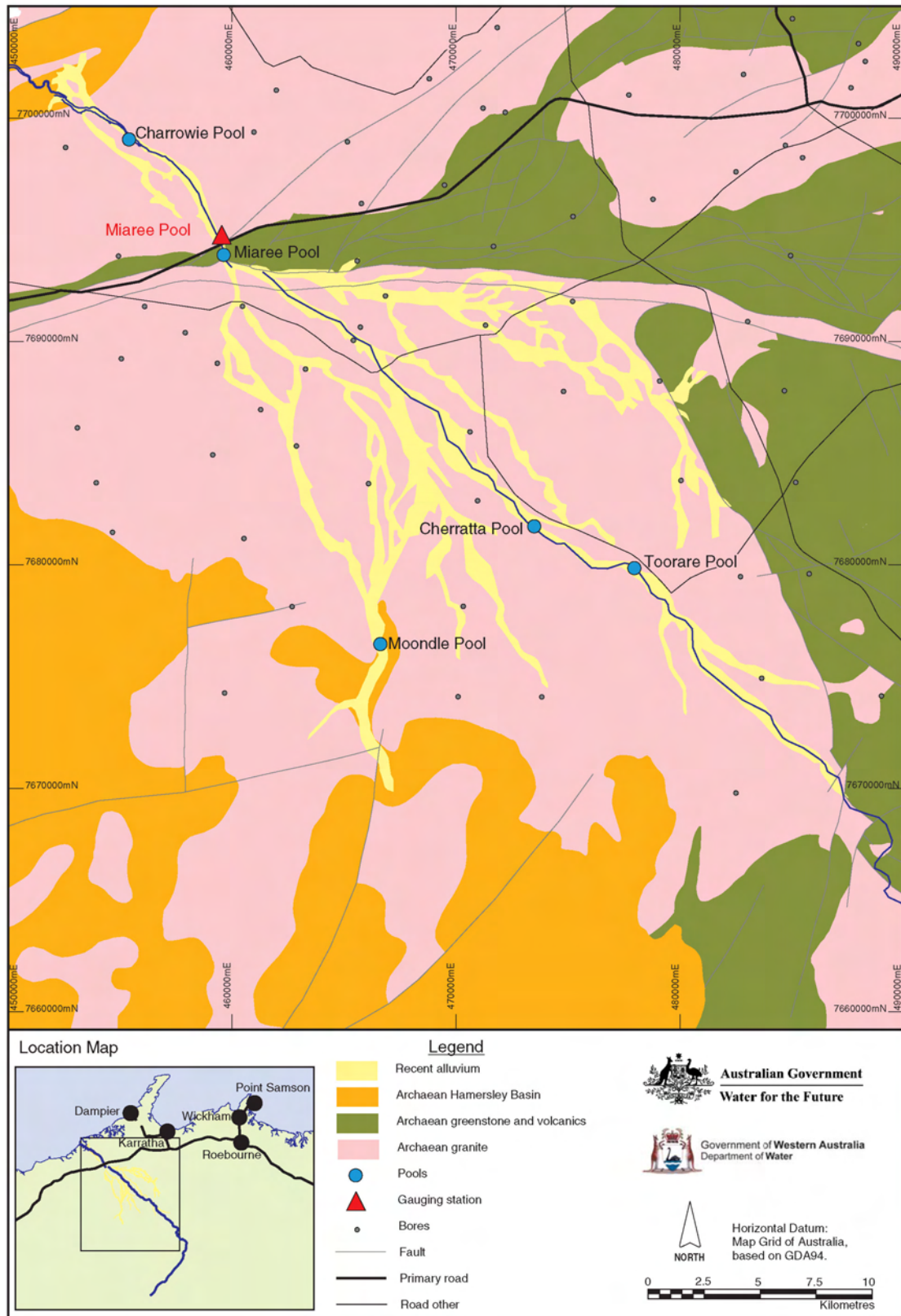
Figure 21: Maitland River Area
