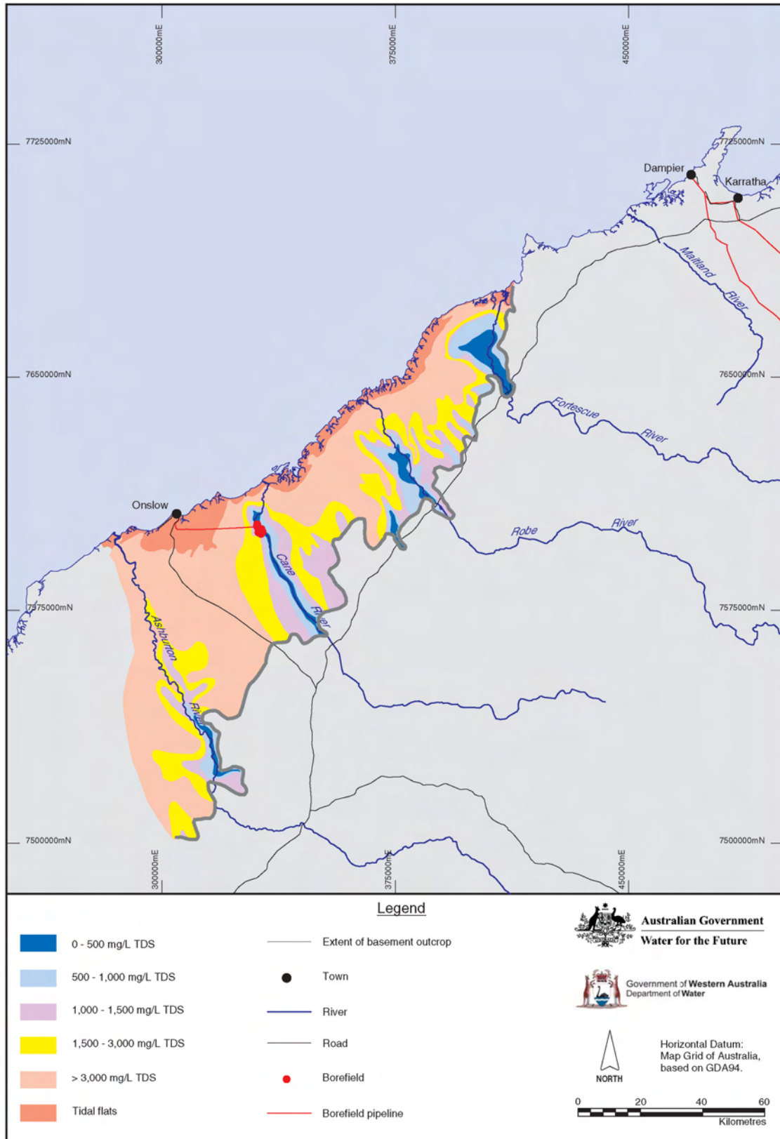
Figure 6: Ashburton Coastal Plain groundwater salinity
