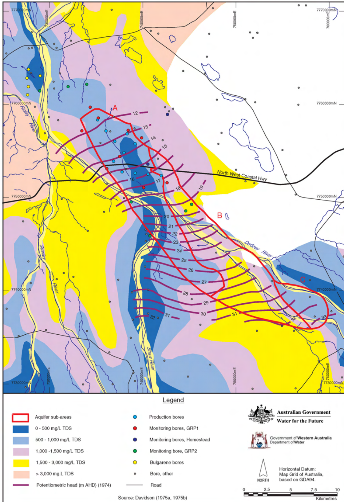
Figure 31: De Grey River salinity
