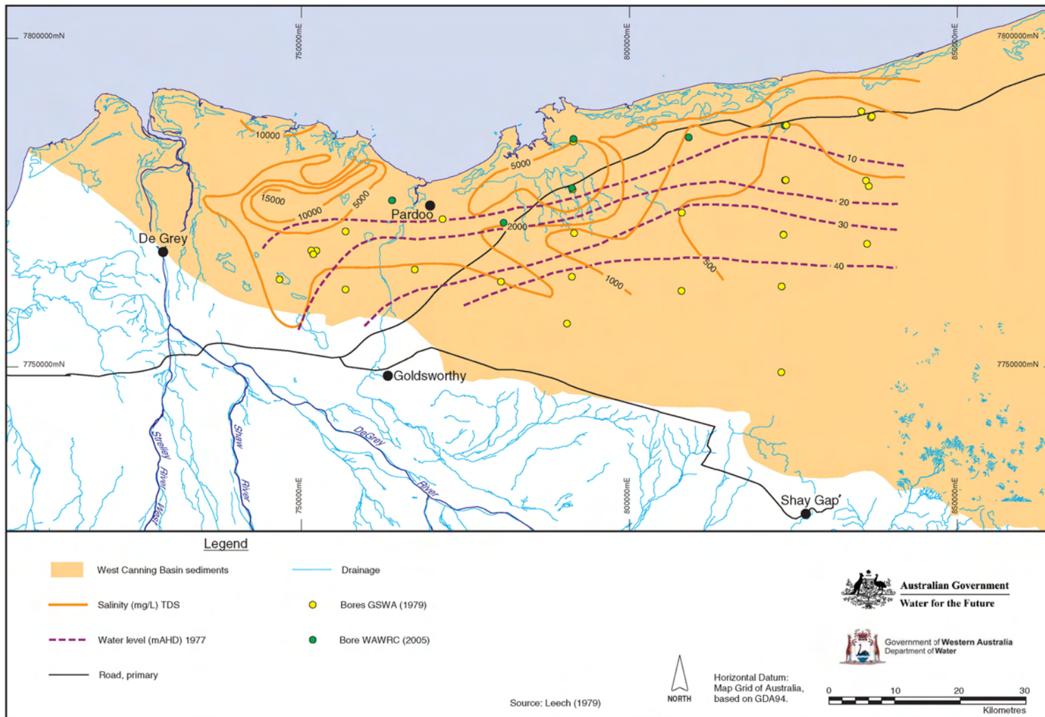
Figure 39: West Canning Basin salinity and water table in the unconfined aquifers
