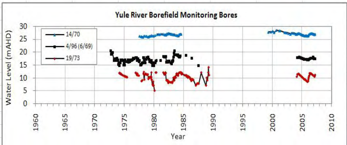
Figure 27: Yule River hydrographs and borefield production
