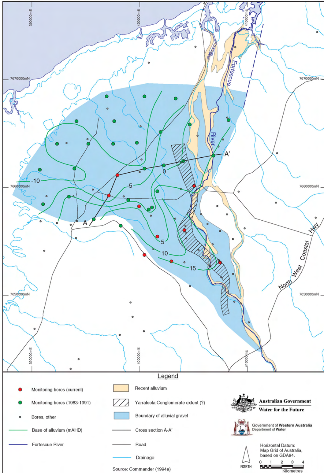
Figure 16: Lower Fortescue River base of alluvium
