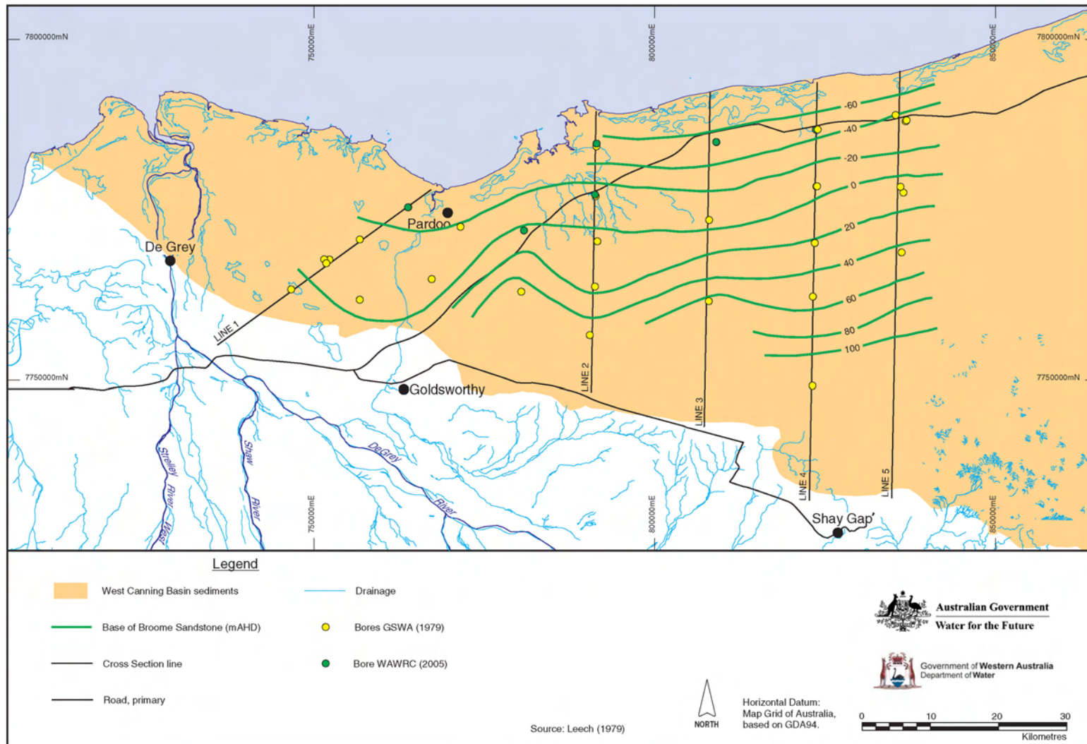
Figure 38: West Canning Basin base of Broome Sandstone
