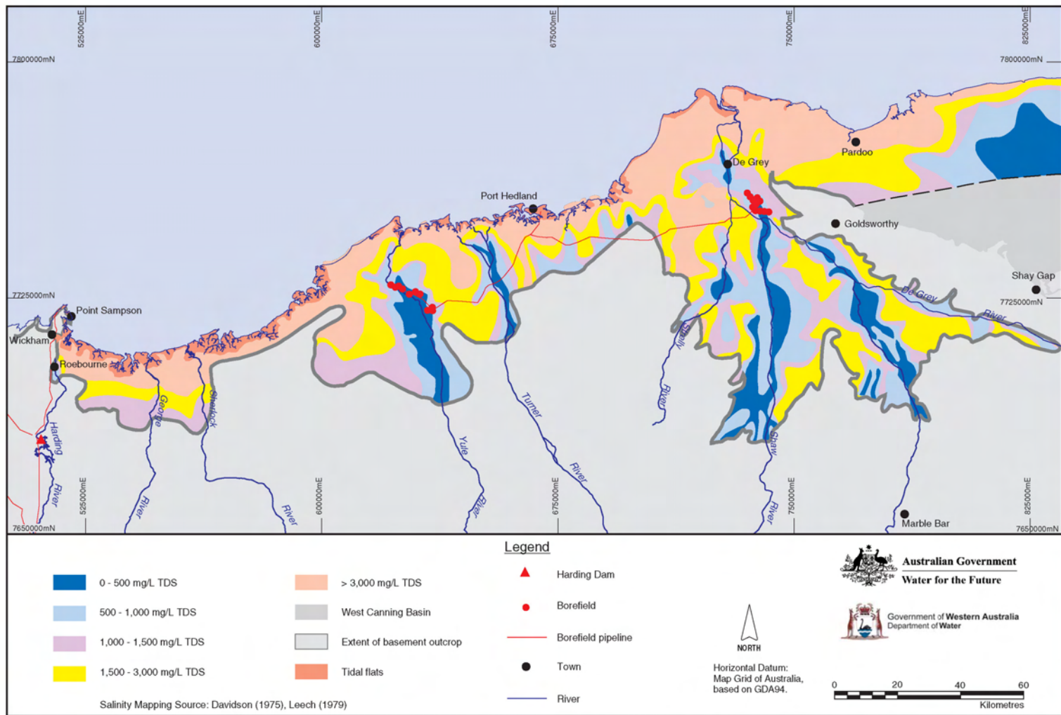
Figure 5: Port Hedland Plain groundwater salinity
