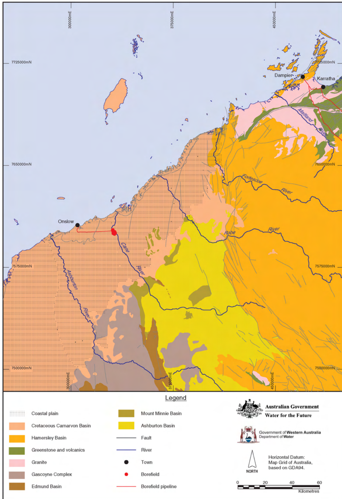
Figure 4: Ashburton Coastal Plain bedrock geology
