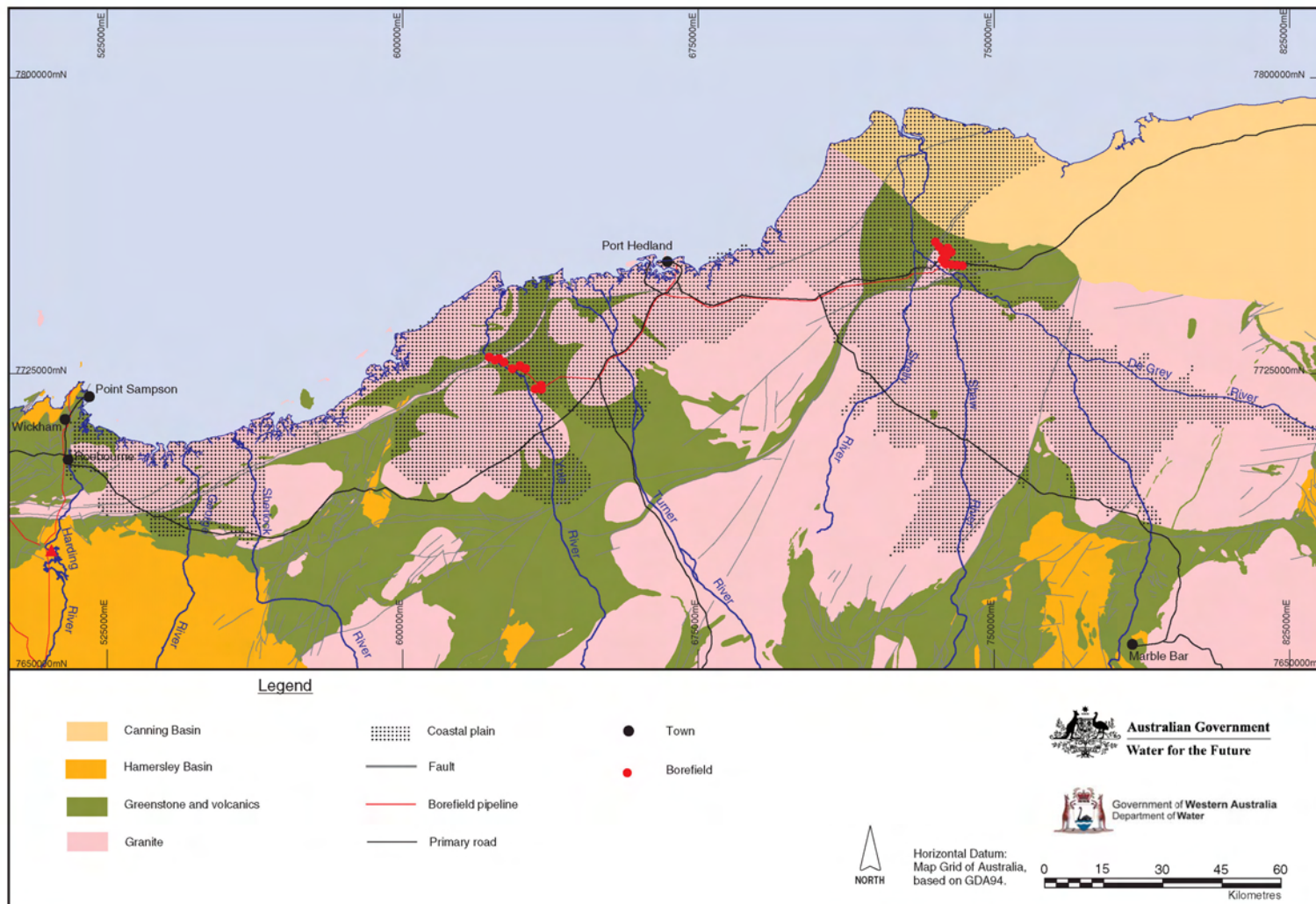
Figure 3: Port Hedland Coastal Plain bedrock geology
