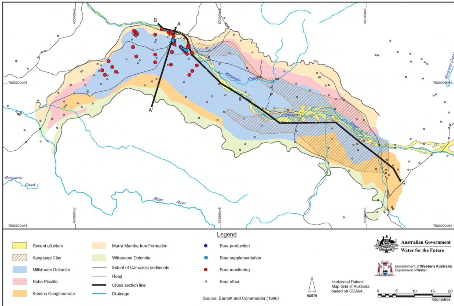
Figure 9: Millstream aquifer
