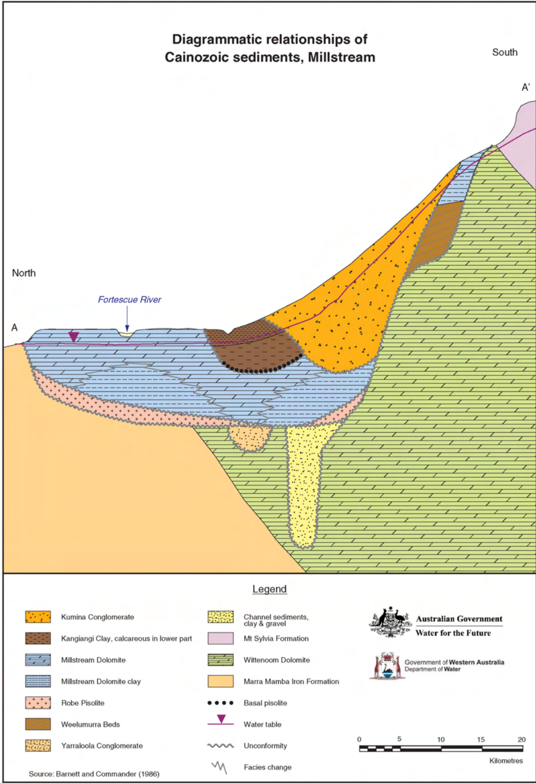
Figure 10: Millstream cross-section, across drainage
