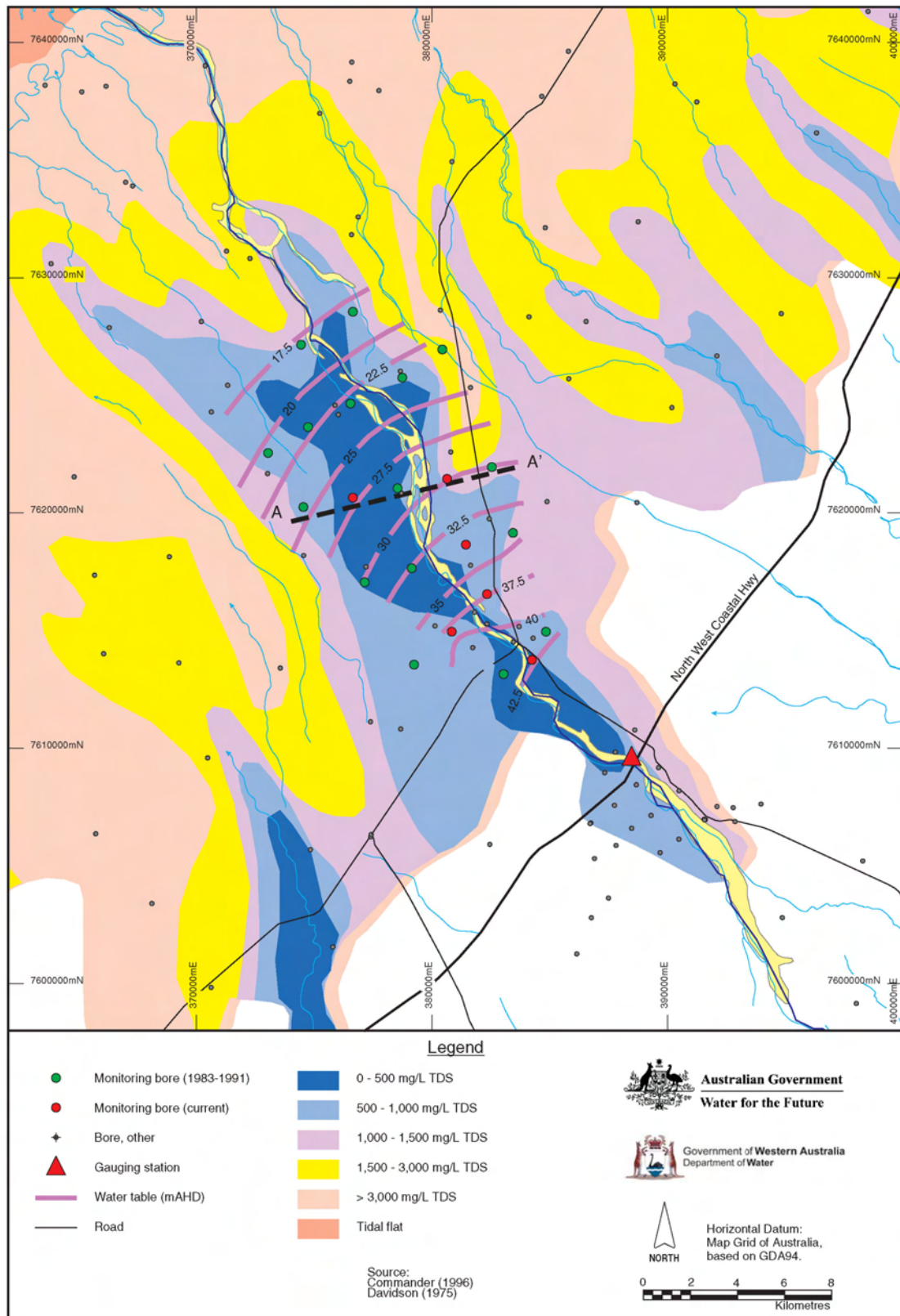
Figure 50: Robe River water levels and salinity
