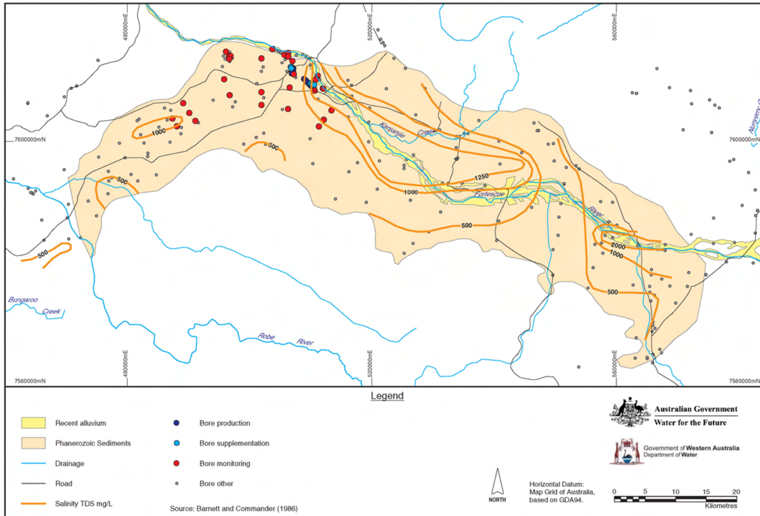
Figure 13: Millstream groundwater salinity in Cainozoic aquifers
