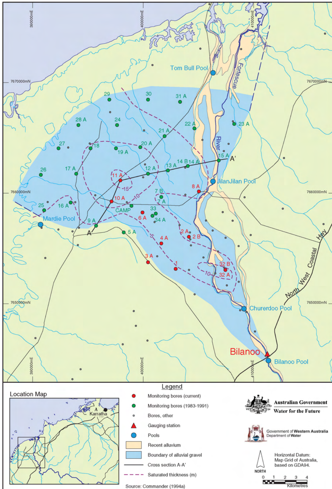
Figure 15: Lower Fortescue River
