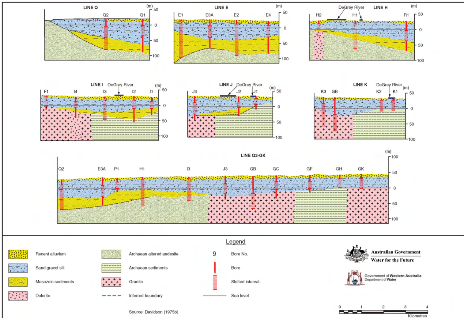
Figure 30: De Grey River cross-sections
