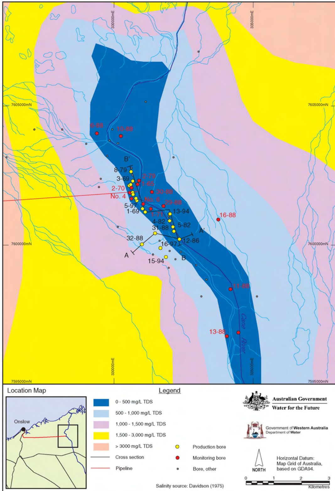
Figure 44: Cane River borefield
