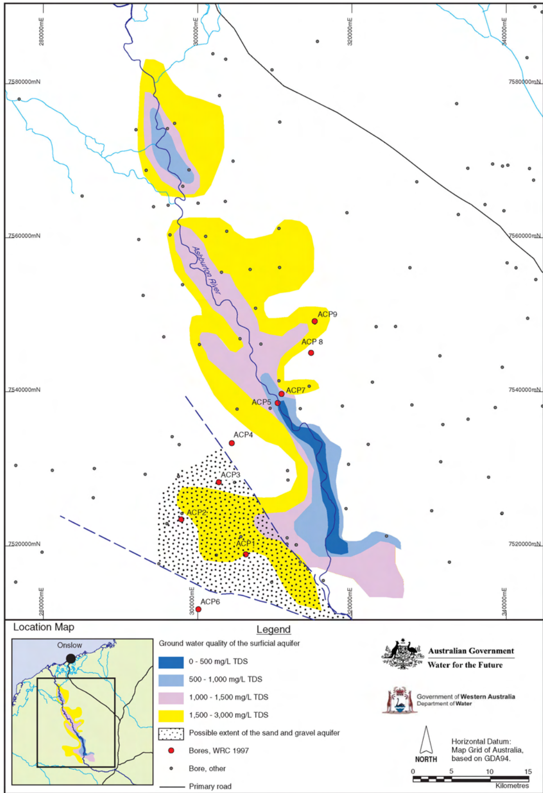
Figure 52: Ashburton River area
