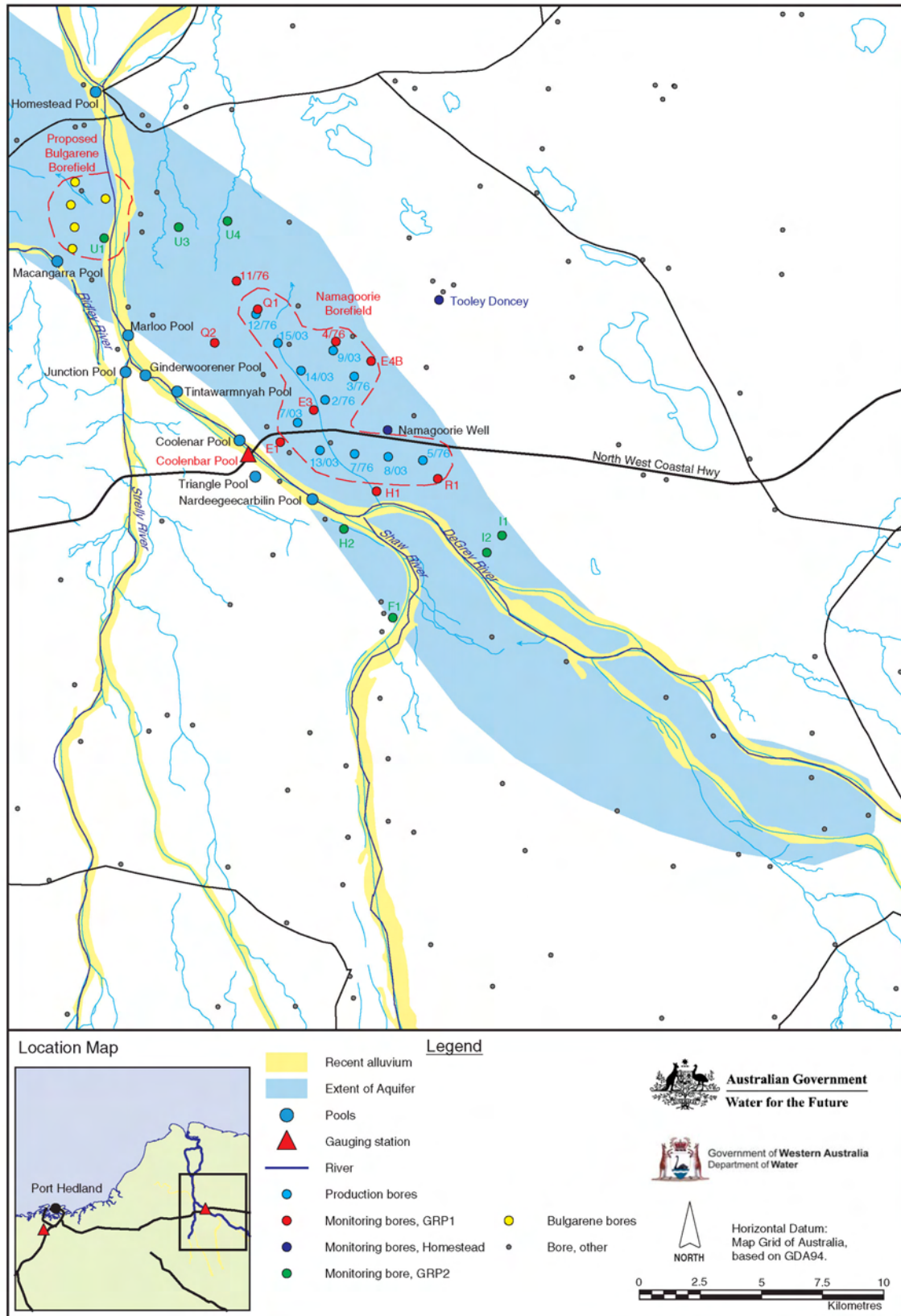
Figure 28: De Grey River borefield
