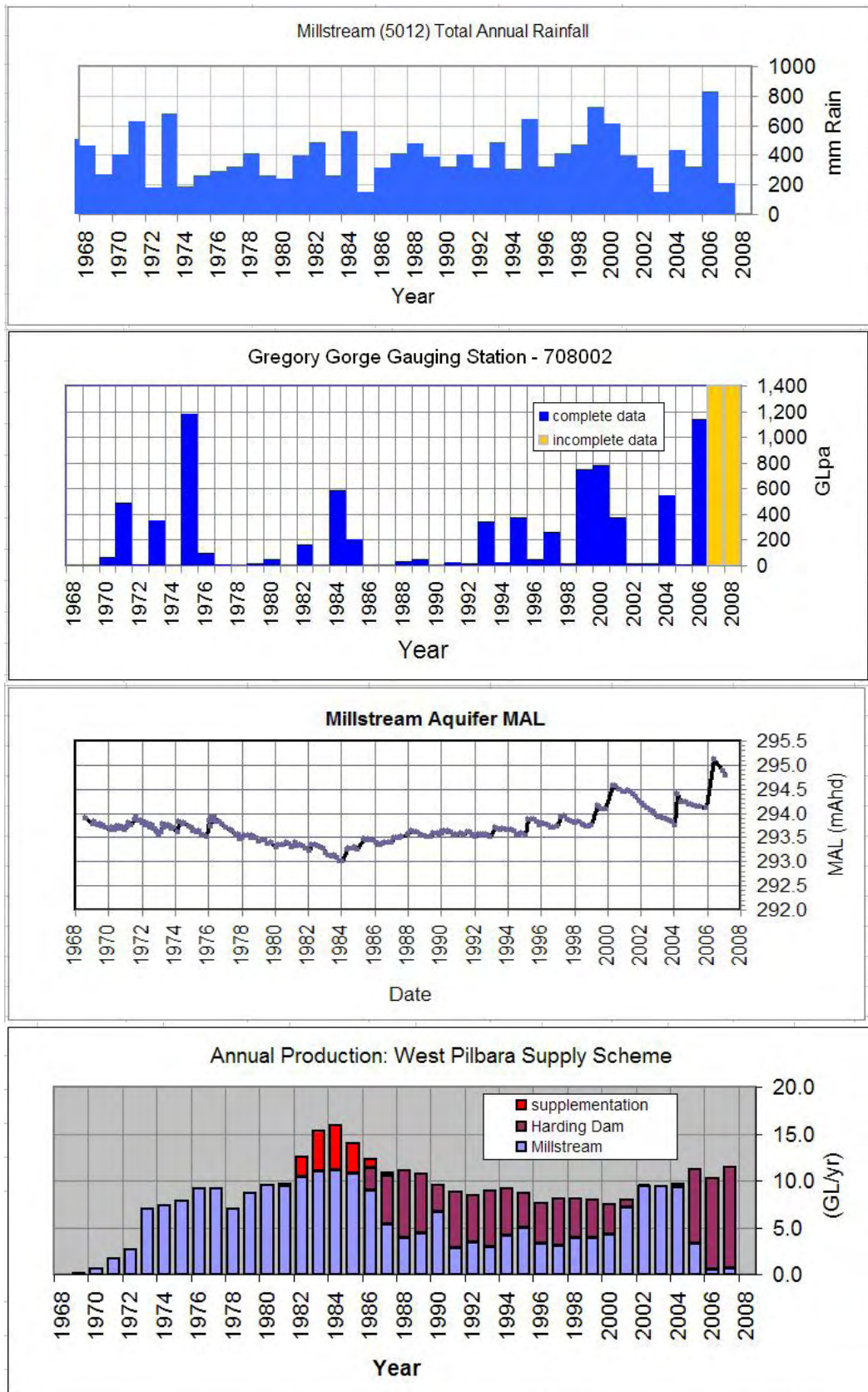
Figure 12: Millstream hydrographs and borefield production
