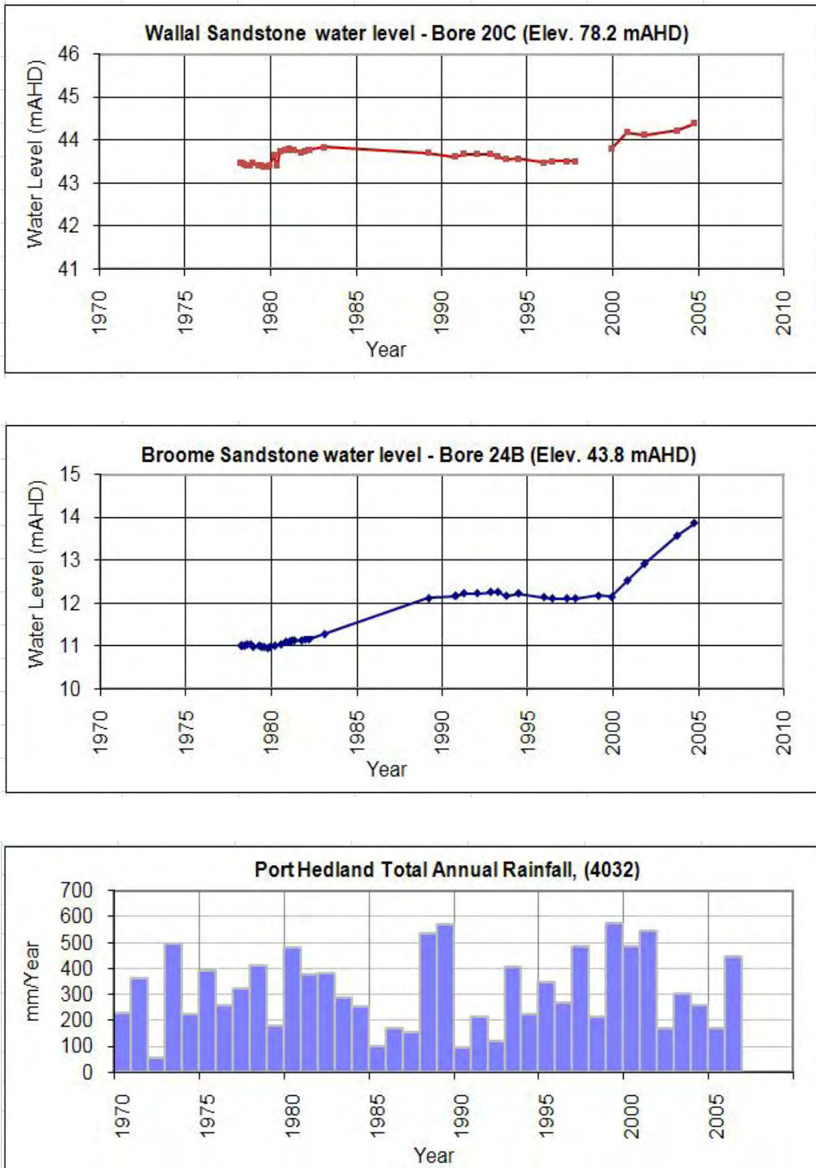
Figure 36: West Canning Basin hydrographs
