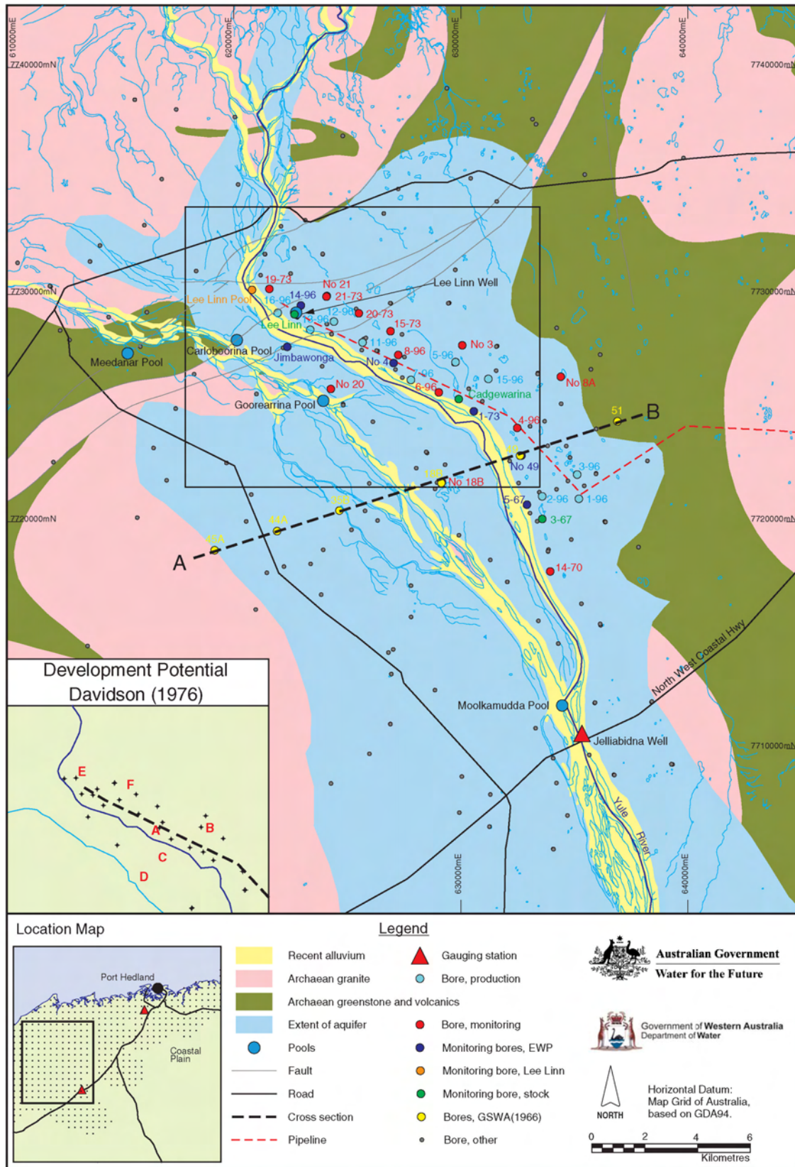
Figure 23: Yule River borefield
