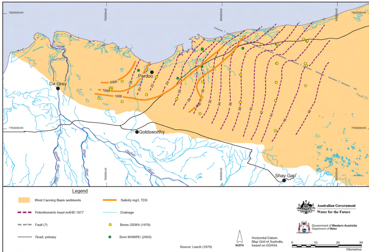
Figure 37: West Canning Basin Wallal aquifer potentiometric surface and salinity
