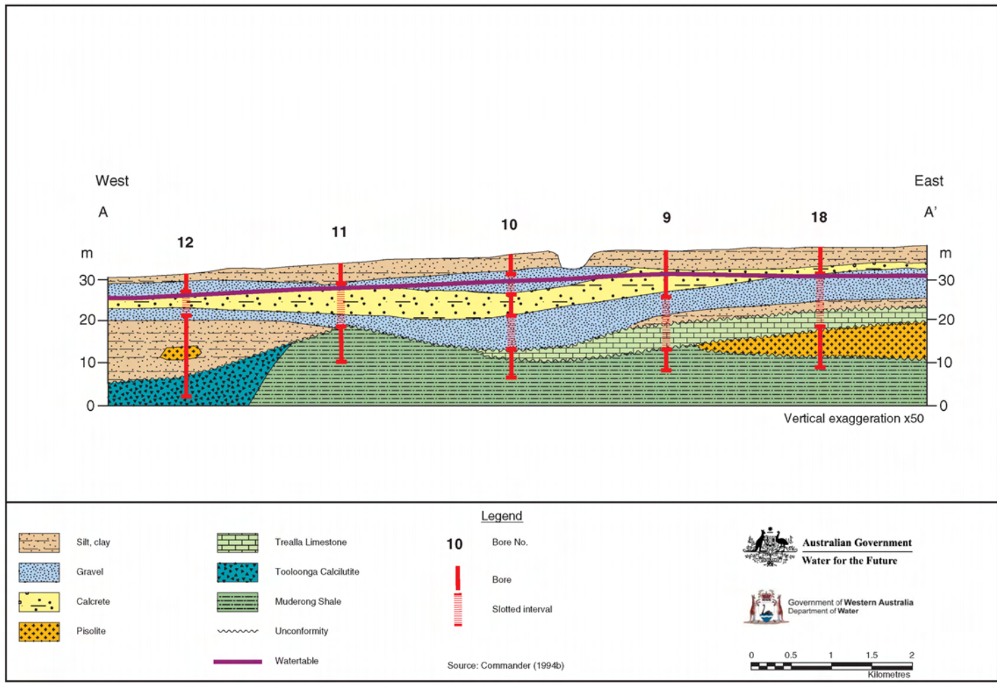
Figure 48: Lower Robe River cross-section A-A'
