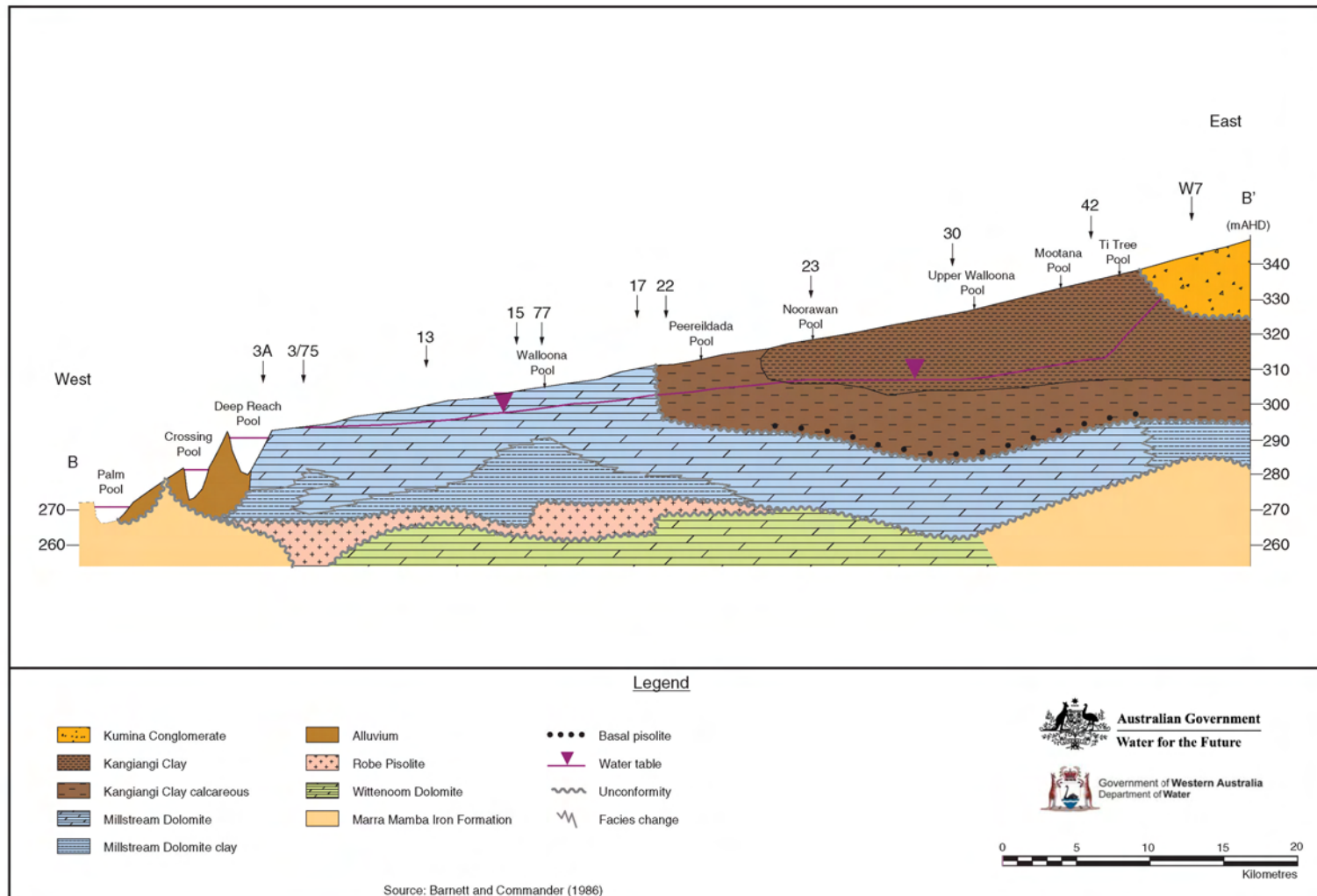
Figure 11: Millstream cross-section, along drainage
