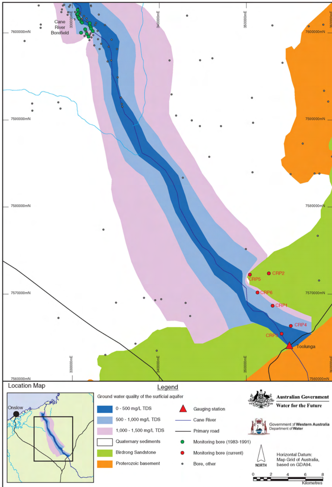
Figure 51: Upper Cane River area
