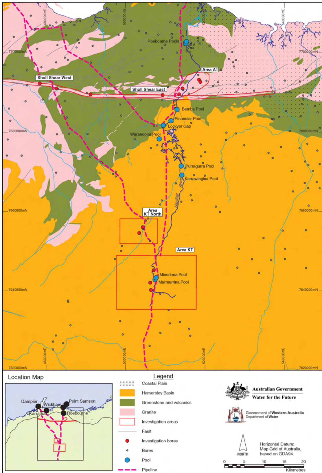
Figure 20: Harding River Area fractured bedrock investigation
