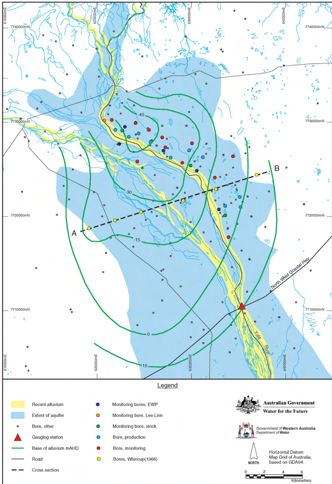
Figure 24: Yule River base of alluvium
