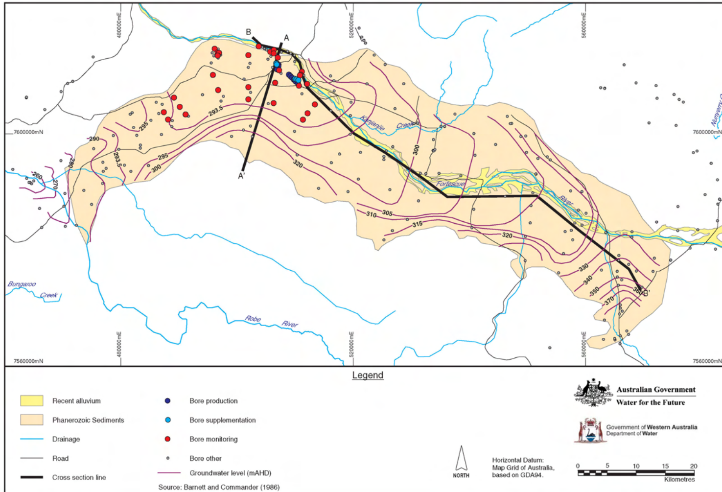
Figure 14: Millstream water levels in the Cainozoic aquifers
