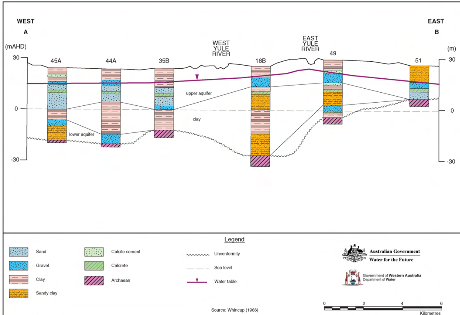
Figure 25: Yule River cross-section A-B
