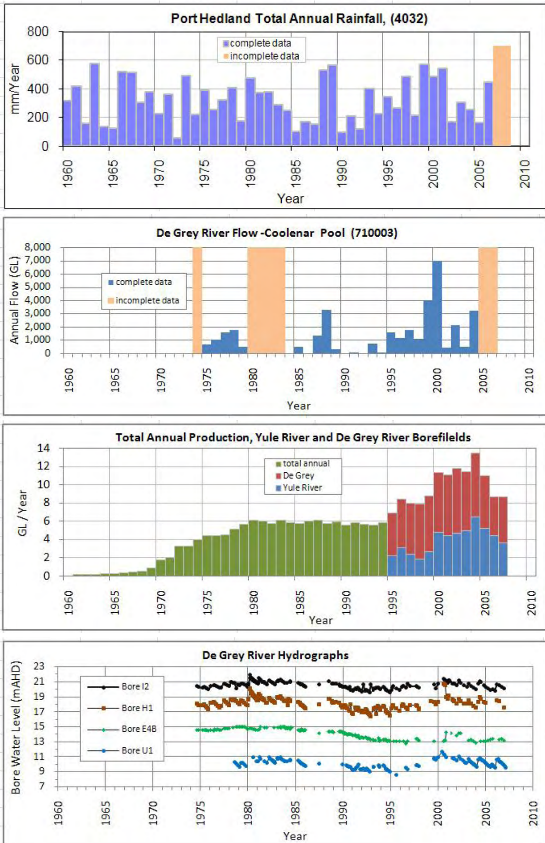
Figure 32: De Grey River hydrographs and borefield production
