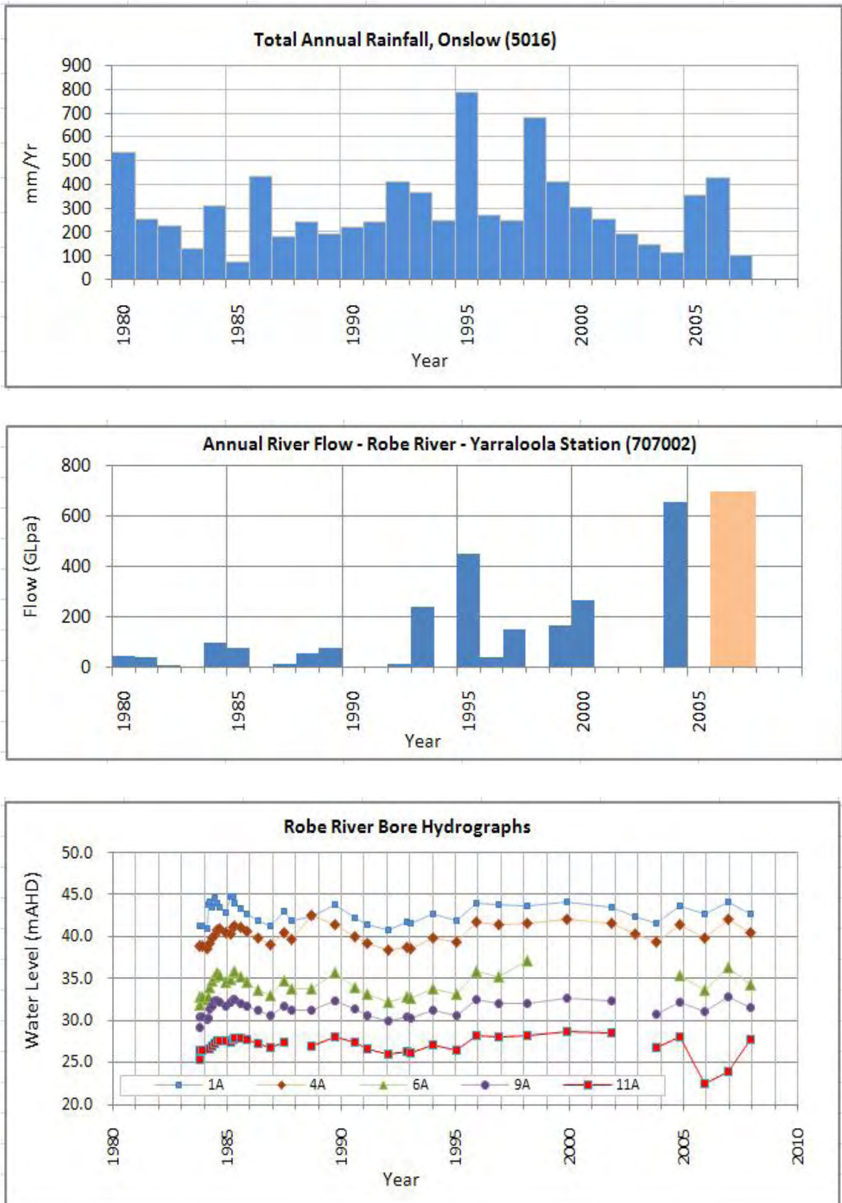
Figure 49: Robe River hydrographs
