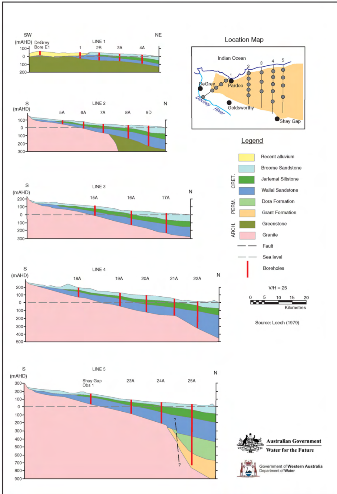
Figure 34: West Canning Basin geological cross-sections
