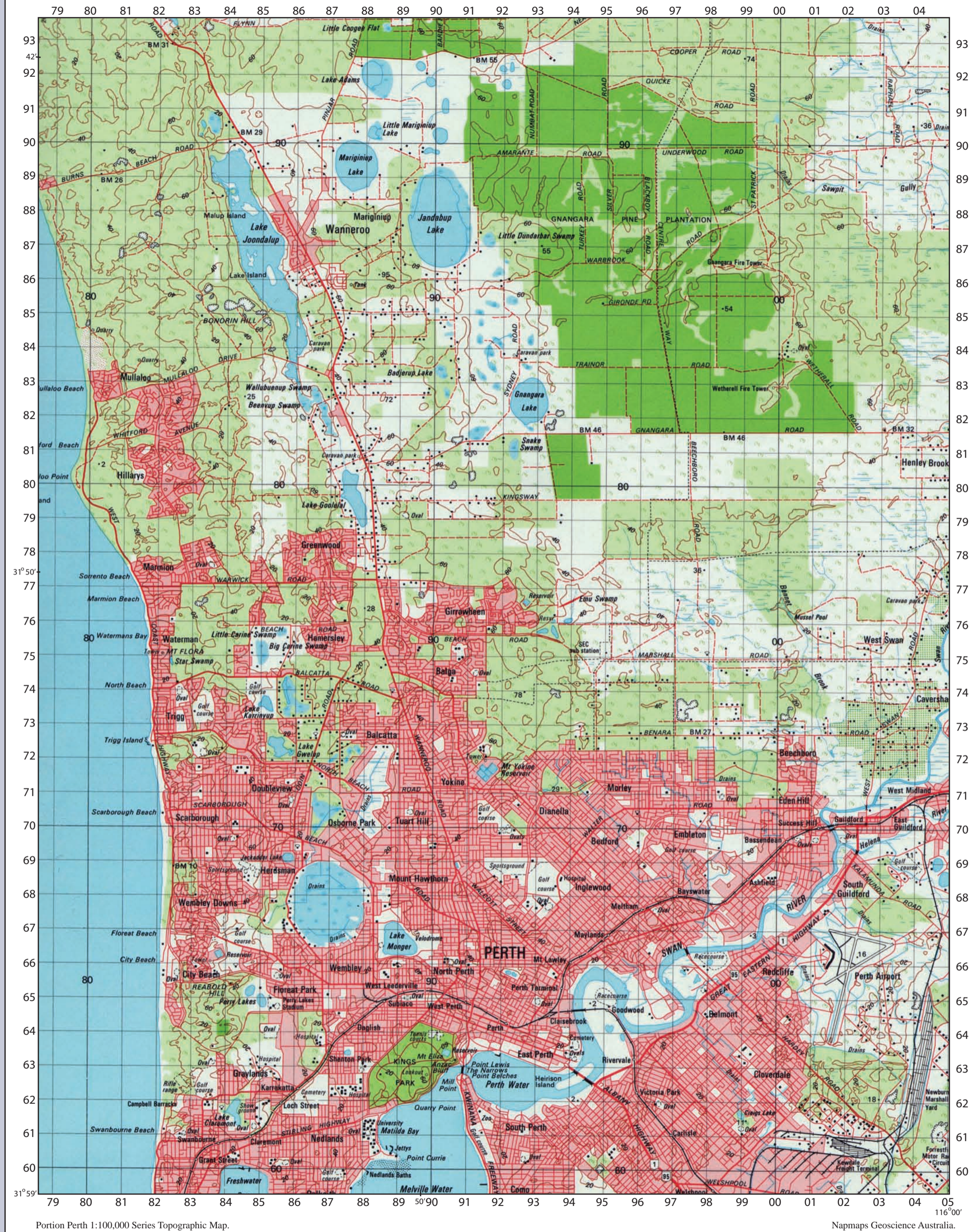
Northern Perth topographic map
