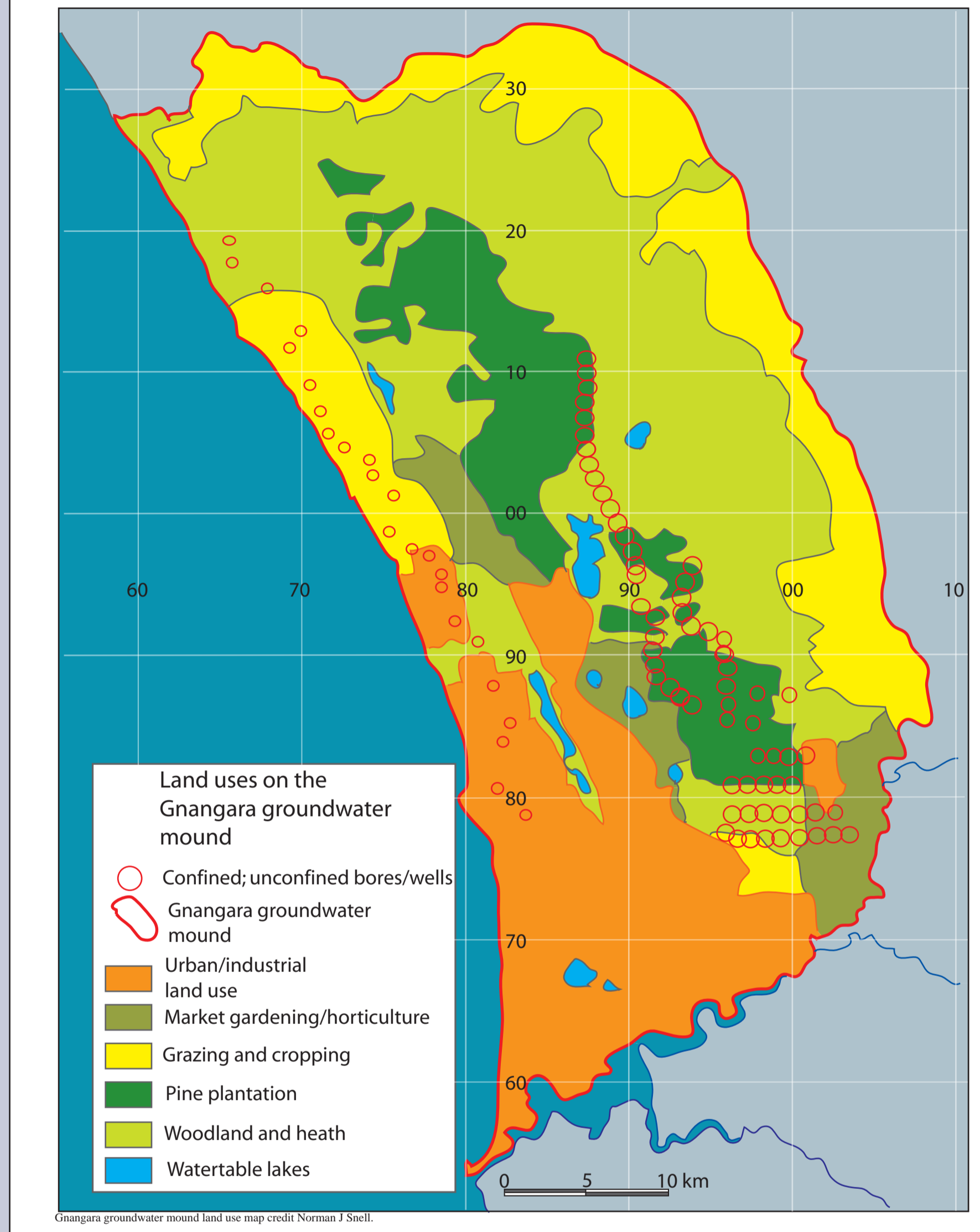
Gnangara groundwater mound - land use map
