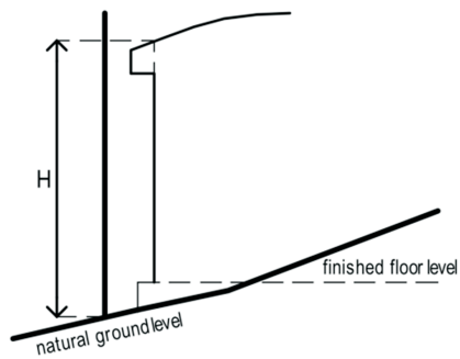
Figure 3d – Cross section, sloped site
