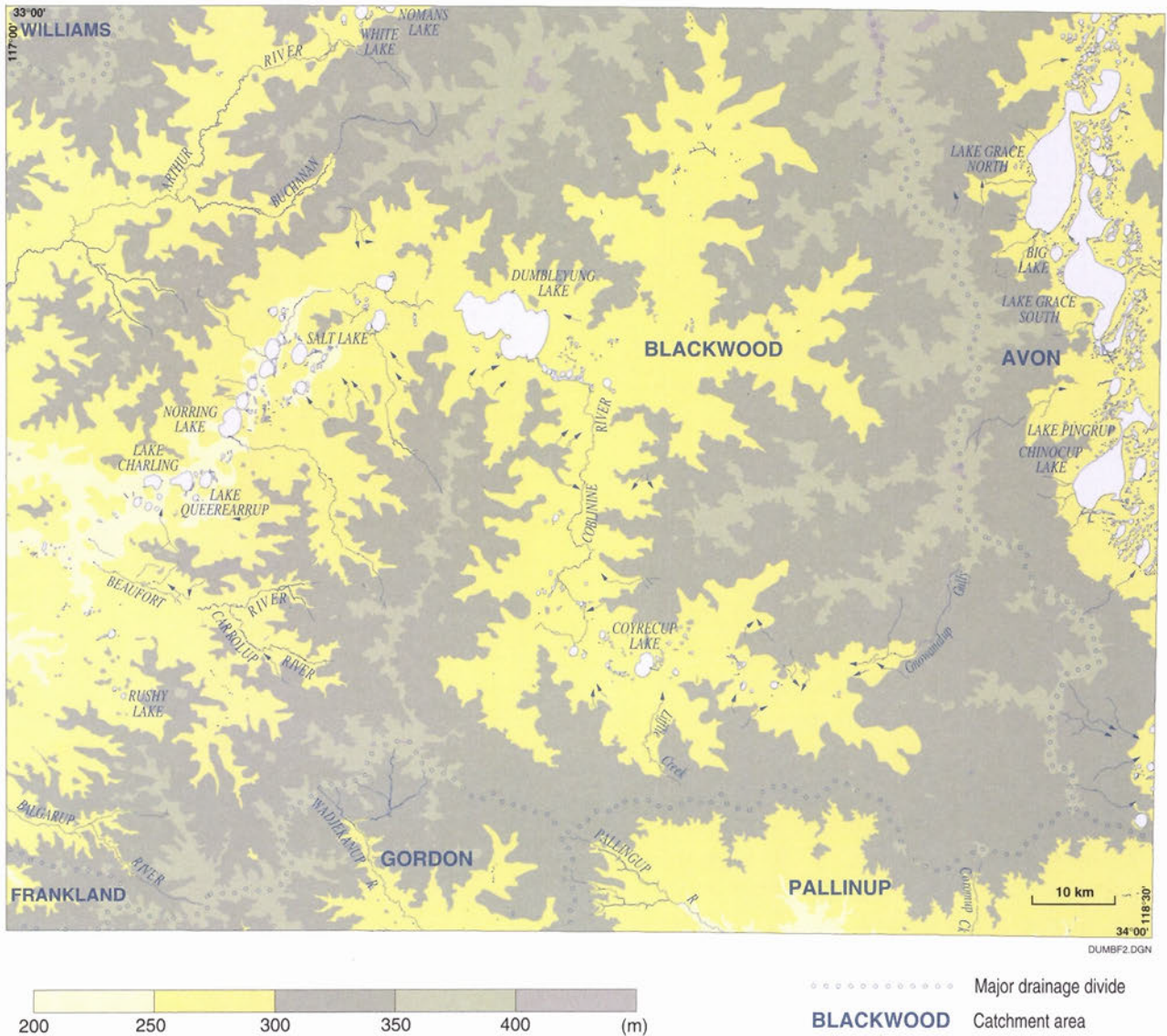
Figure 2. Topography
