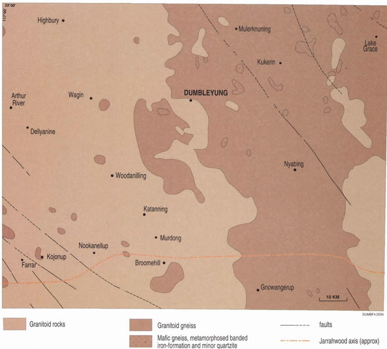
Figure 4. Geological structure
