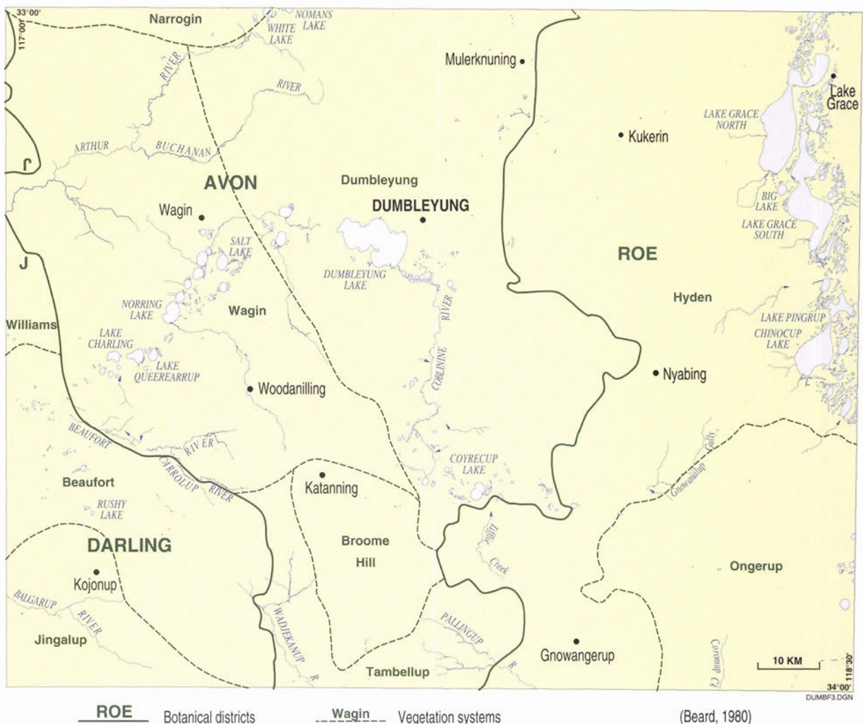
Figure 3. Vegetation systems
