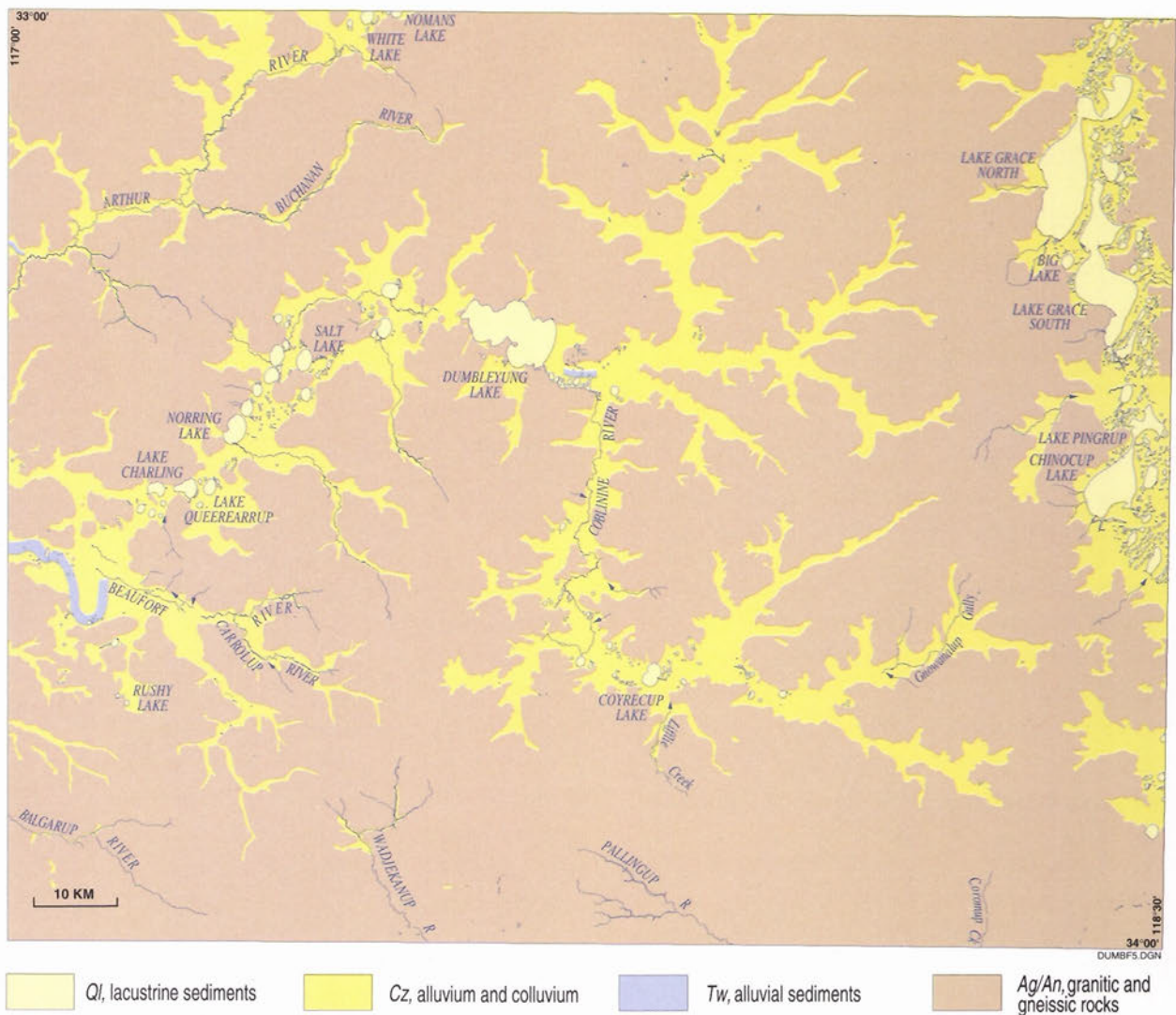
Figure 5. Palaeodrainage systems
