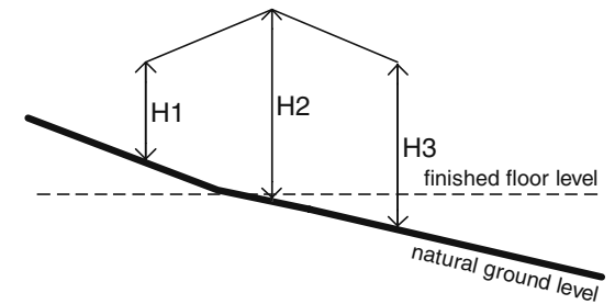
Figure 5c – Elevation – sloped site
