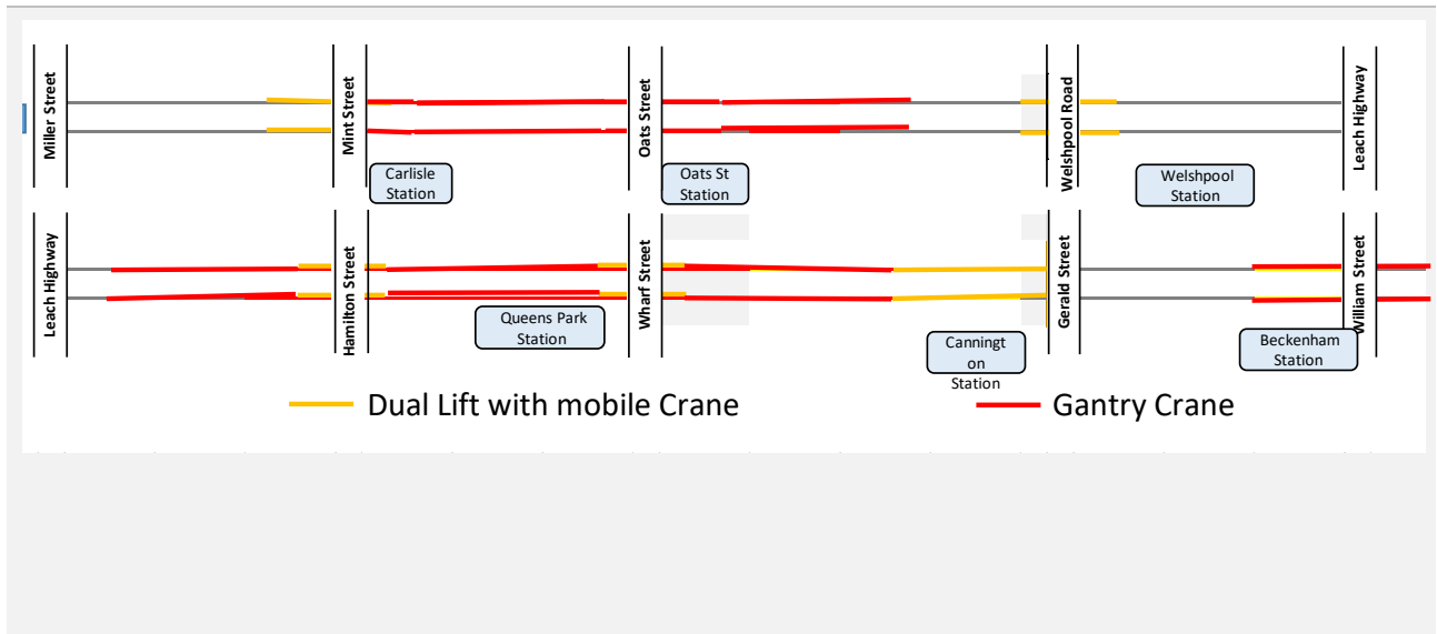
Gantry Crane L-beam lifts
