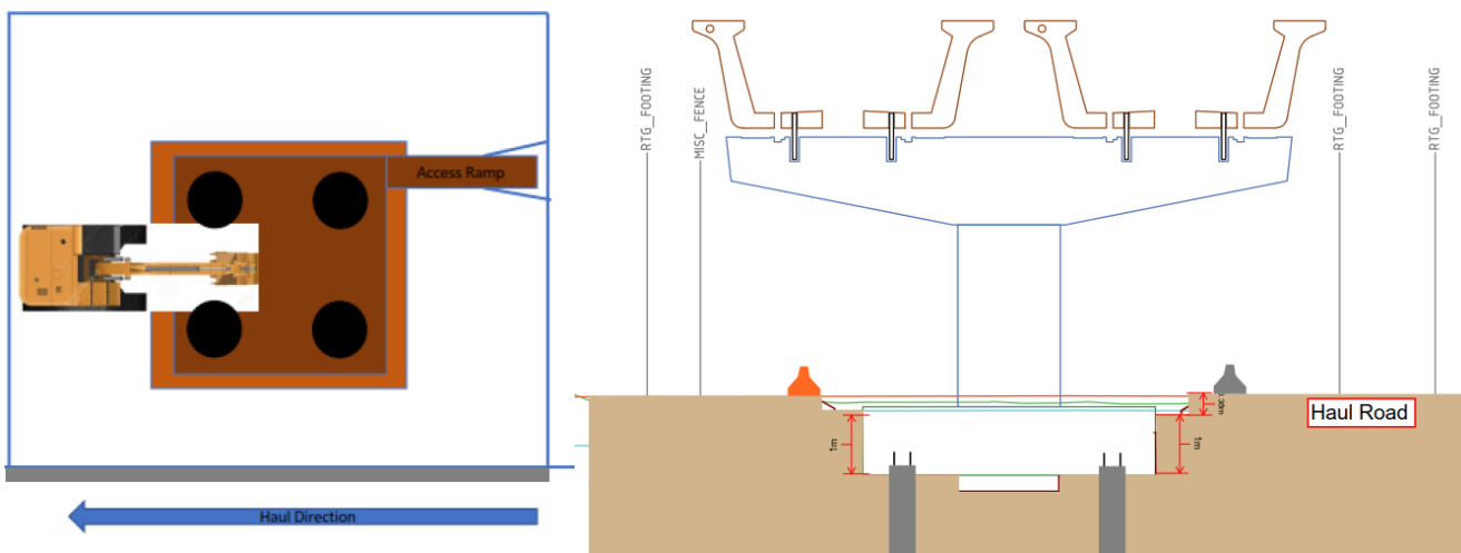
FIGURE 100: EXCAVATION EXTENT
