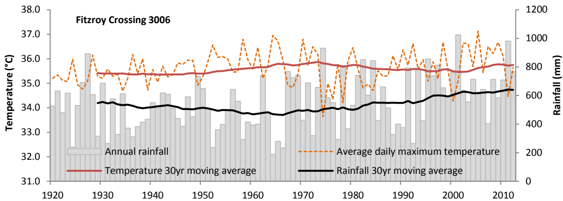
Figure 1-11: Annual rainfall and average daily maximum temperature, 1920–2012 for the Fitzroy Crossing meteorological station (3006) in Kimberley region
