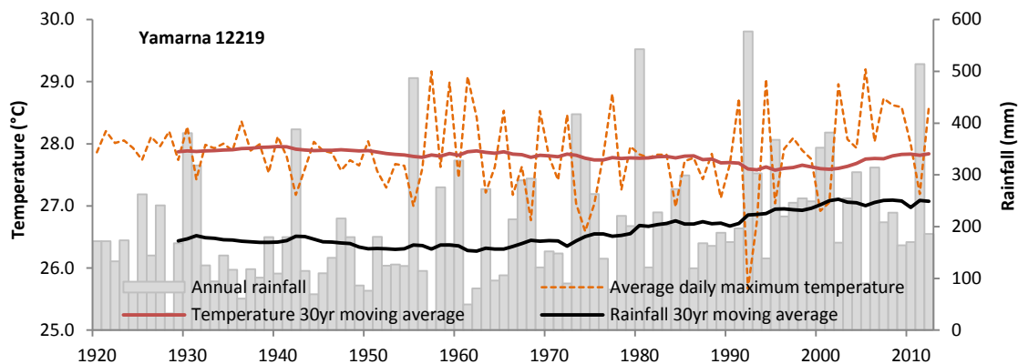
Figure 1-13: Annual rainfall and average daily maximum temperature, 1920–2012 for the Yamarna meteorological station (12219) in the Central region
