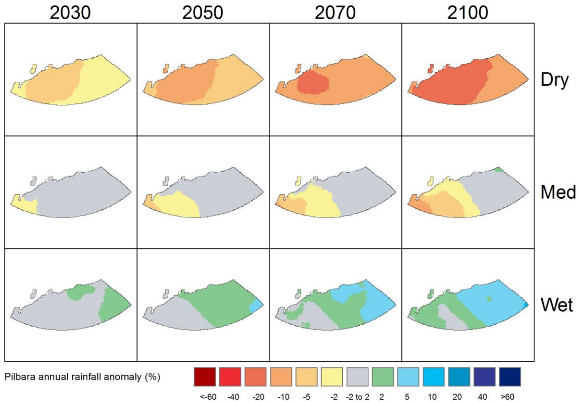
Figure 3-4: Change in average annual rainfall relative to the baseline period for Pilbara region for representative wet, median and dry scenarios at future time horizons
