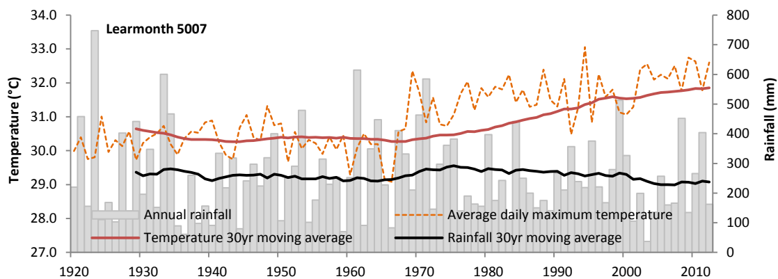
Figure 1-10: Annual rainfall and average daily maximum temperature, 1920–2012 for the Learmonth Airport meteorological station (5007) in Pilbara region
