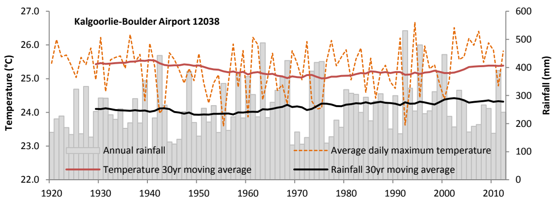
Figure 1-12: Annual rainfall and average daily maximum temperature, 1920–2012 for the Kalgoorlie meteorological station (12038) in the Central region
