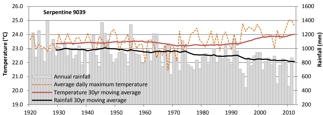
Figure 1-7: Annual rainfall and average daily maximum temperature, 1920–2012 for the Serpentine meteorological station (9039) in the South-west region
