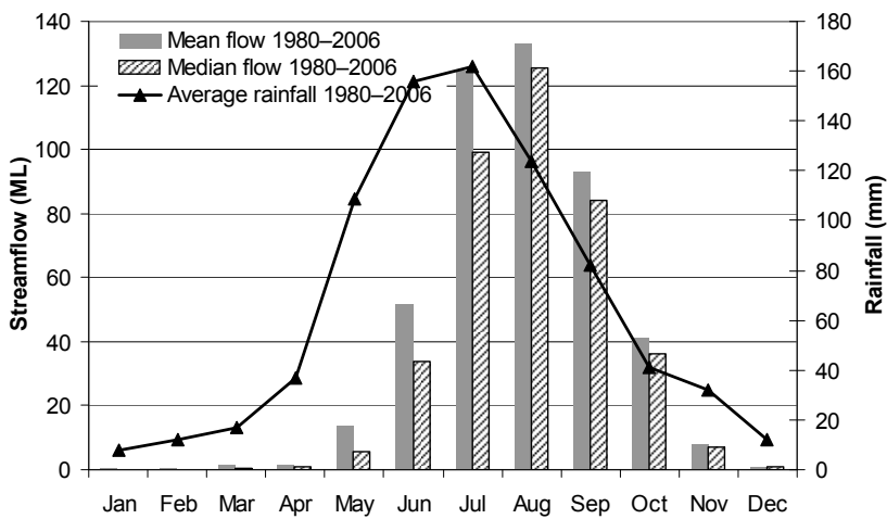
Figure 35: Dugalup Brook modelled monthly flow 1980—2006.
