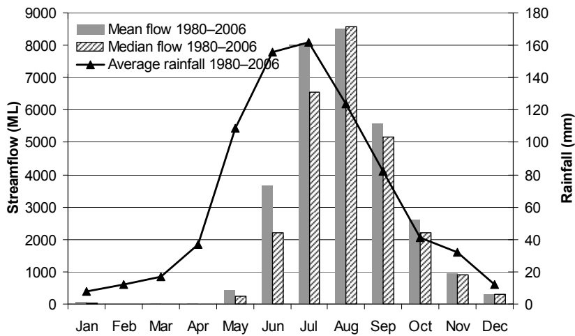
Figure 37: Carburnup River modelled monthly flow 1980–2006.
