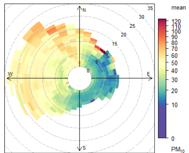
Figure 2 Polar plot from November 2019 to August 2020 showing the higher concentrations of PM 10 originating from the western (ocean) side of the site (yellow-orange portion of plot) indicating the likely influence of marine aerosols (sea salt)
