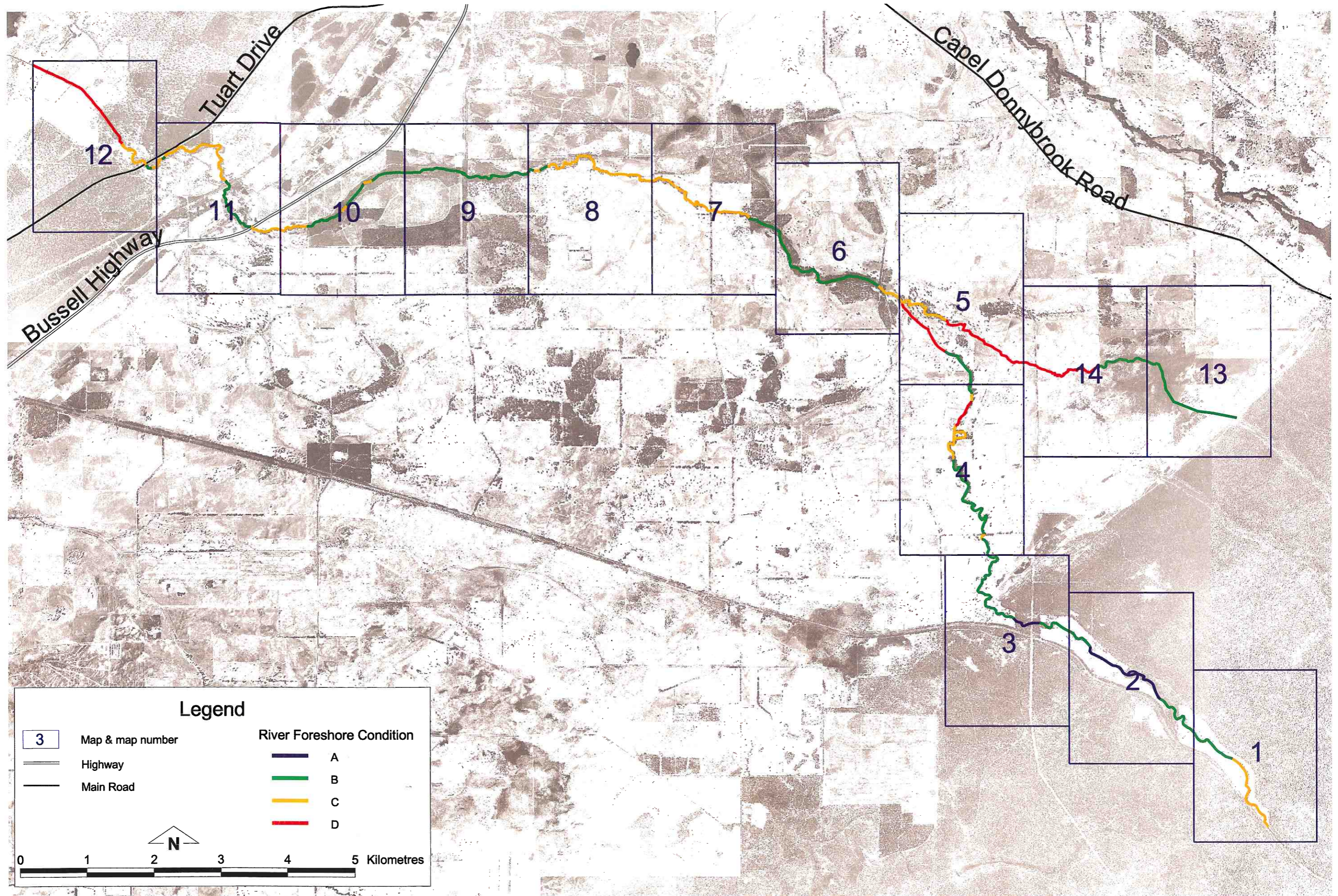
Figure 11: Index map for locating sections of the Ludlow River and Tiger Gully. Map also shows foreshore condition.
