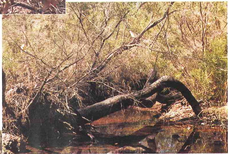
A2 grade foreshore on the upper Sabina River. Fringing vegetation shades the water, providing a cooler environment for aquatic fauna and limiting algal growth.
