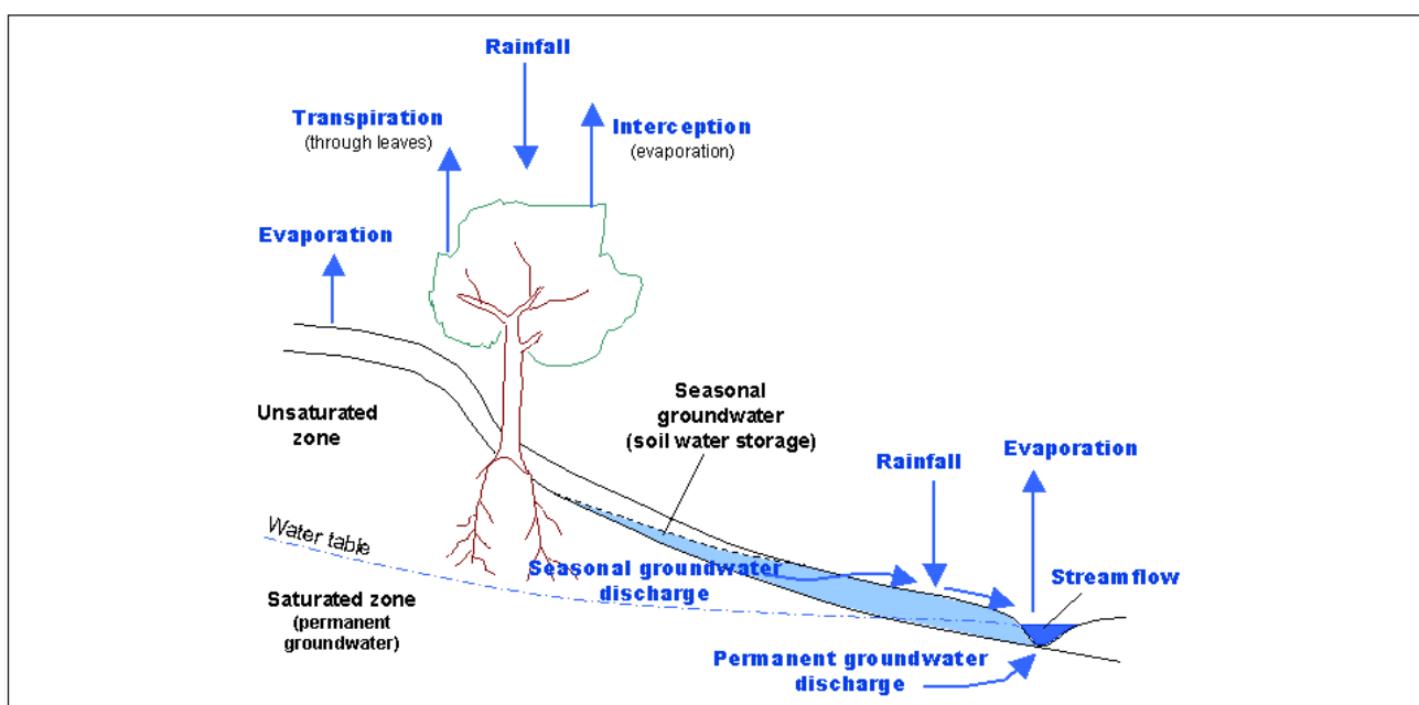
Figure 9. The land-based hydrologic balance.
