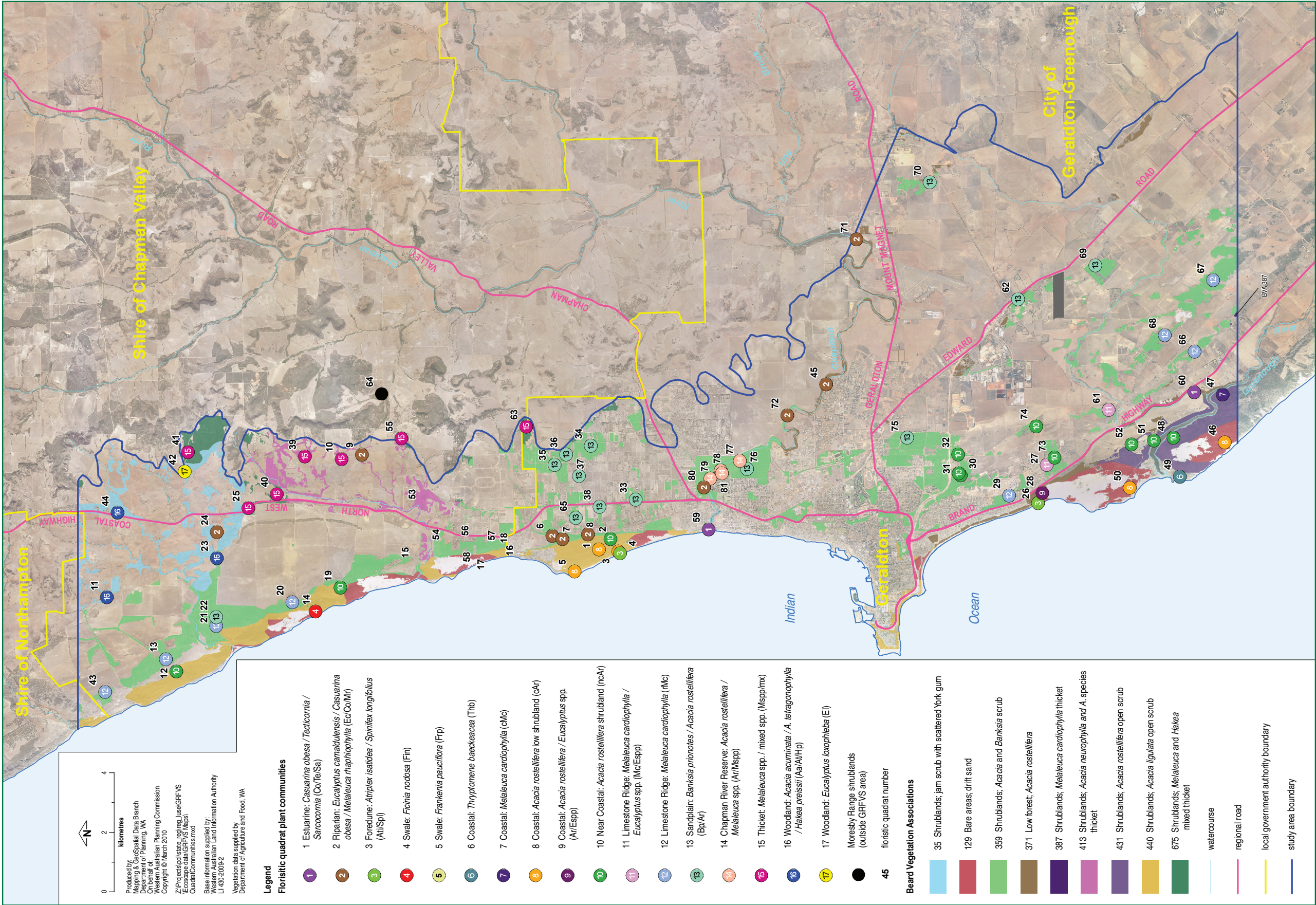
Map 7: Floristic quadrat plant communities and Beard vegetation associations
