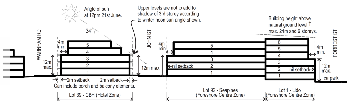
Diagram 7. North-South section through Cottesloe Beach Hotel / Seapines / Lido sites
