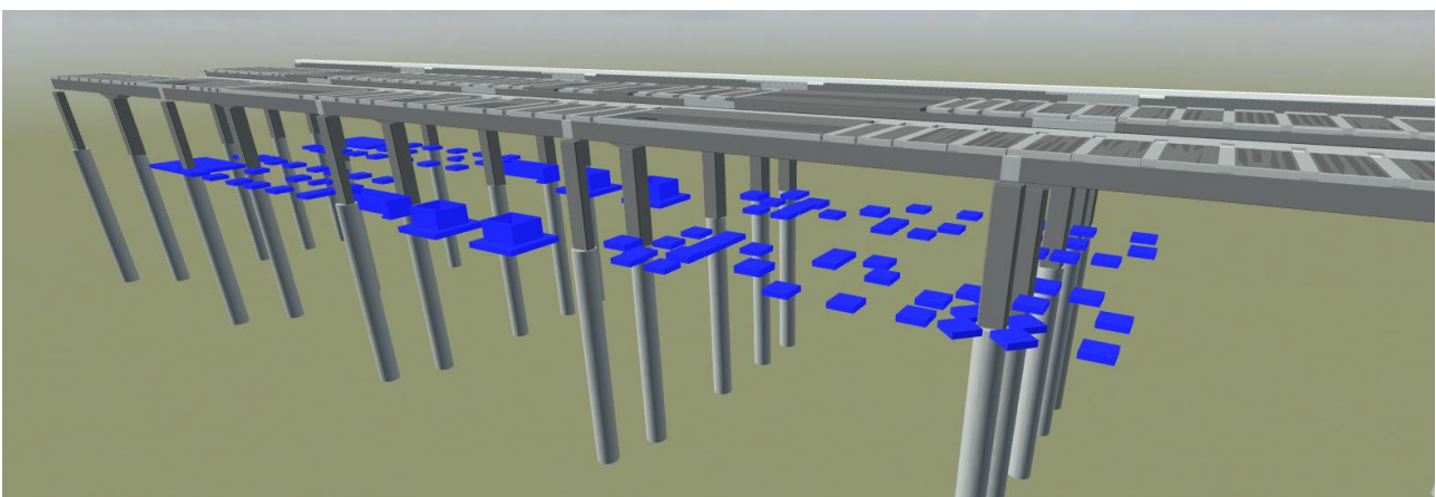
Figure 4: In-Ground Foundations
