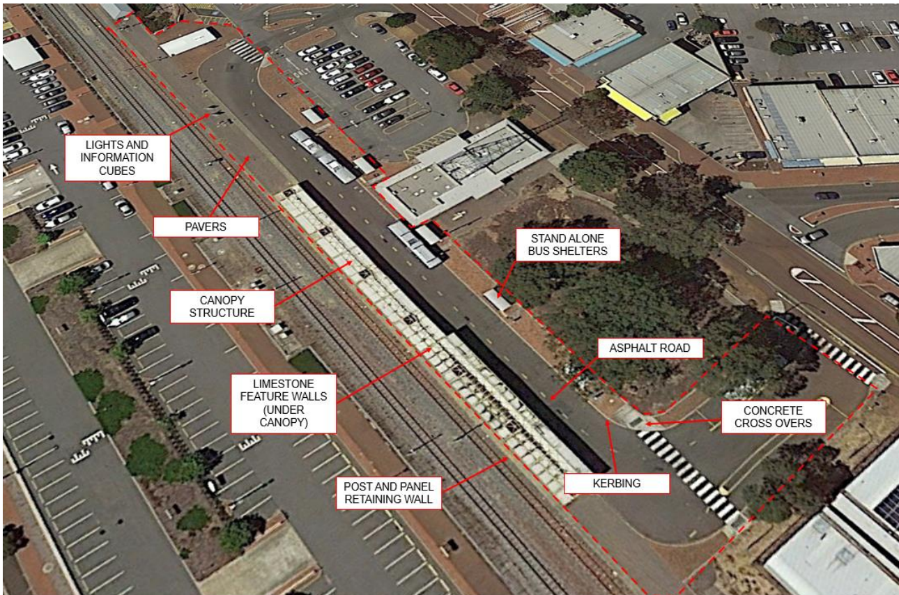
Figure 6: Armadale Bus Interchange Demolition Areas
