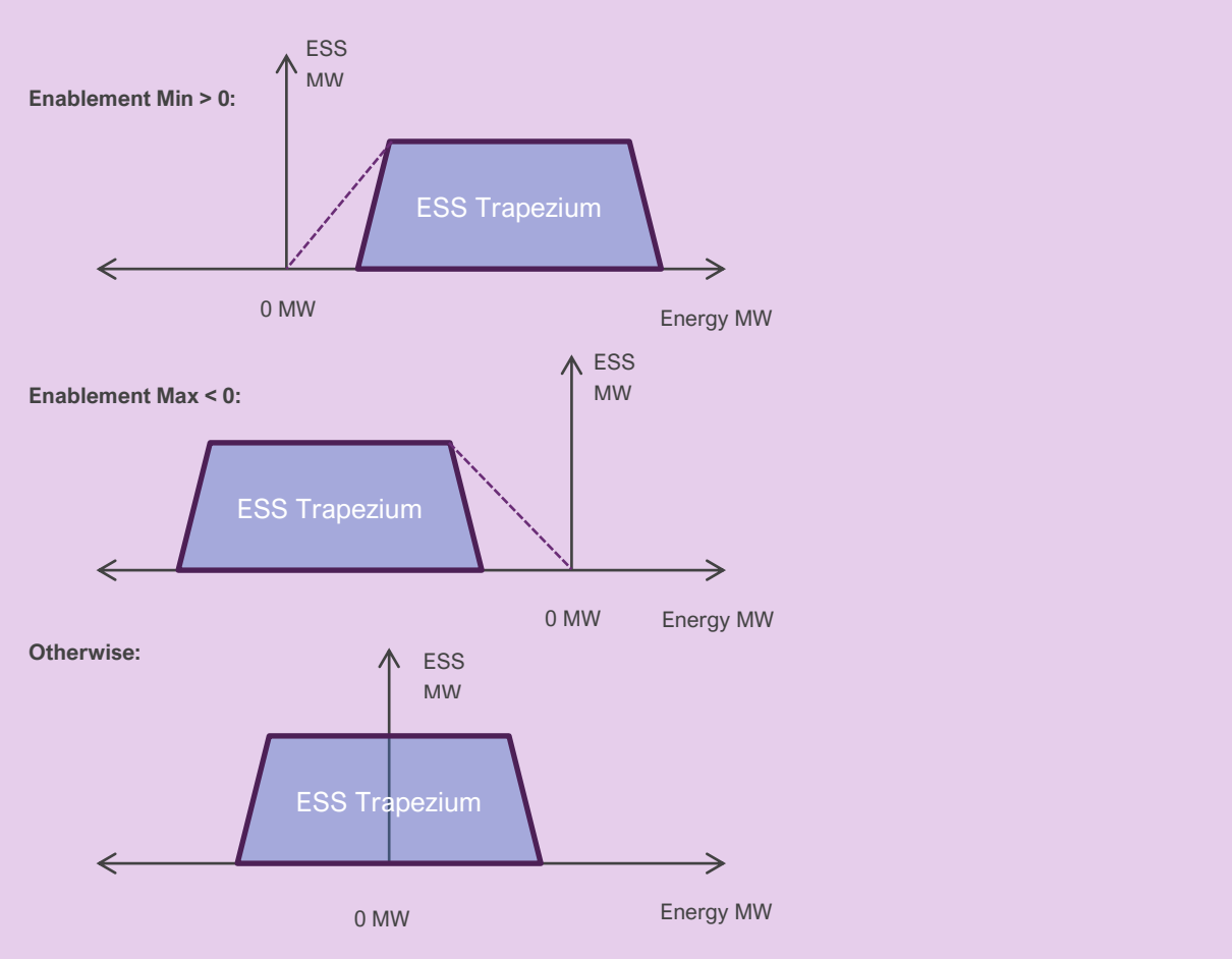
Figure E[2]. Trapezia adjustments for RoCoF Control Service
