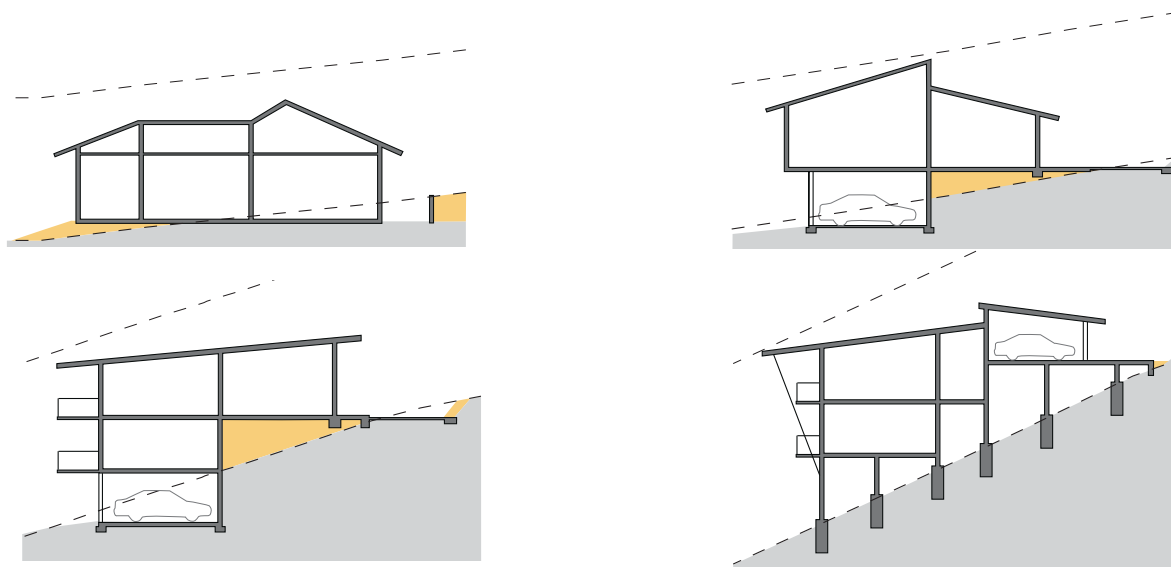
Figure G3.2a Building height for sloping sites
