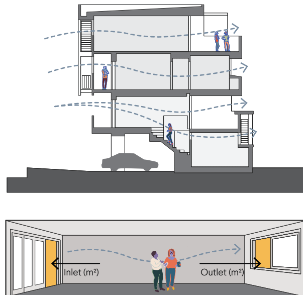
Figure G2.2a Natural ventilation for passive cooling
