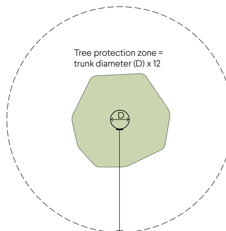
Figure G1.2a Establishing a tree protection zone
