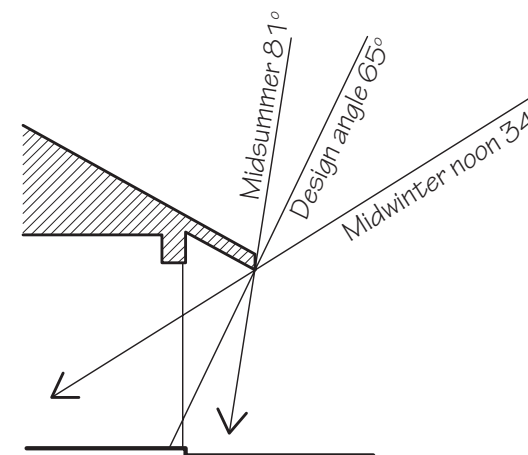
Figure 70 Calculated eaves overhang on north side, Perth
