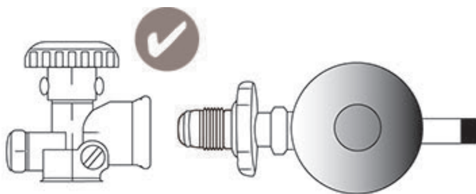
POL valve + POL regulator connection
