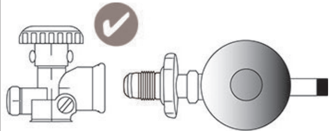
POL valve + POL regulator connection
