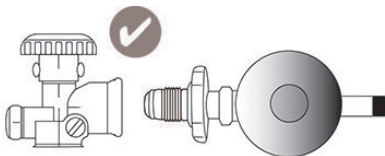
POL valve + POL regulator connection
