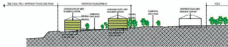
EAST - WEST SITE SECTION SECTION A - A
