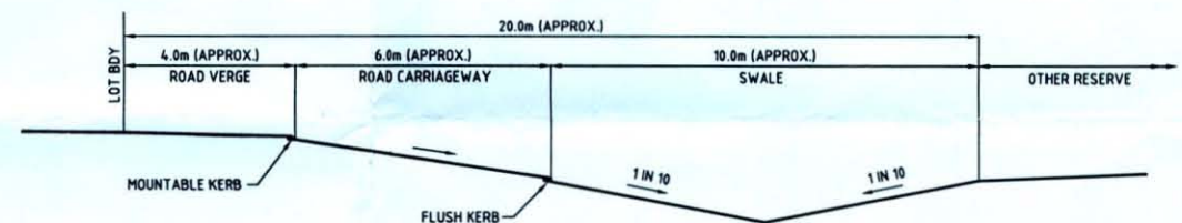
DETAIL A - TYPICAL CROSS-SECTION THROUGH ROADS EAST AND WEST OF SUB-CATCHMENTS 1 AND 3 NOT TO SCALE
