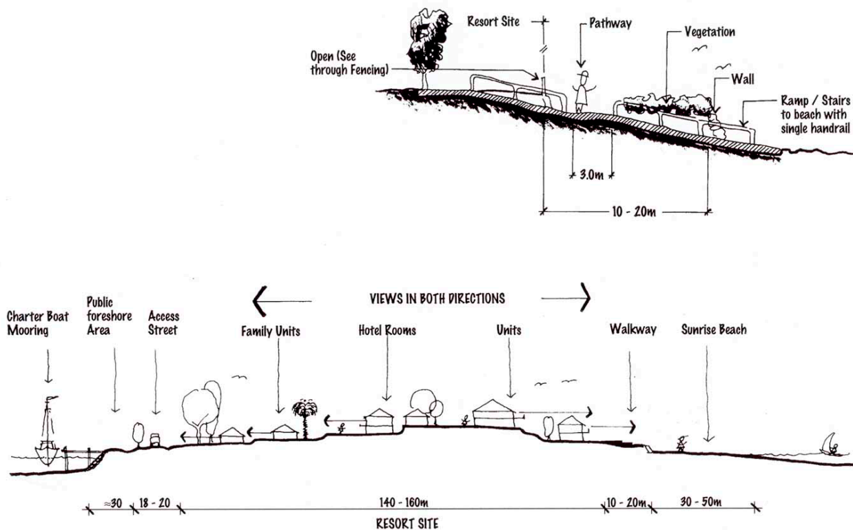
Figure 8: Precinct C Typical Cross-section
