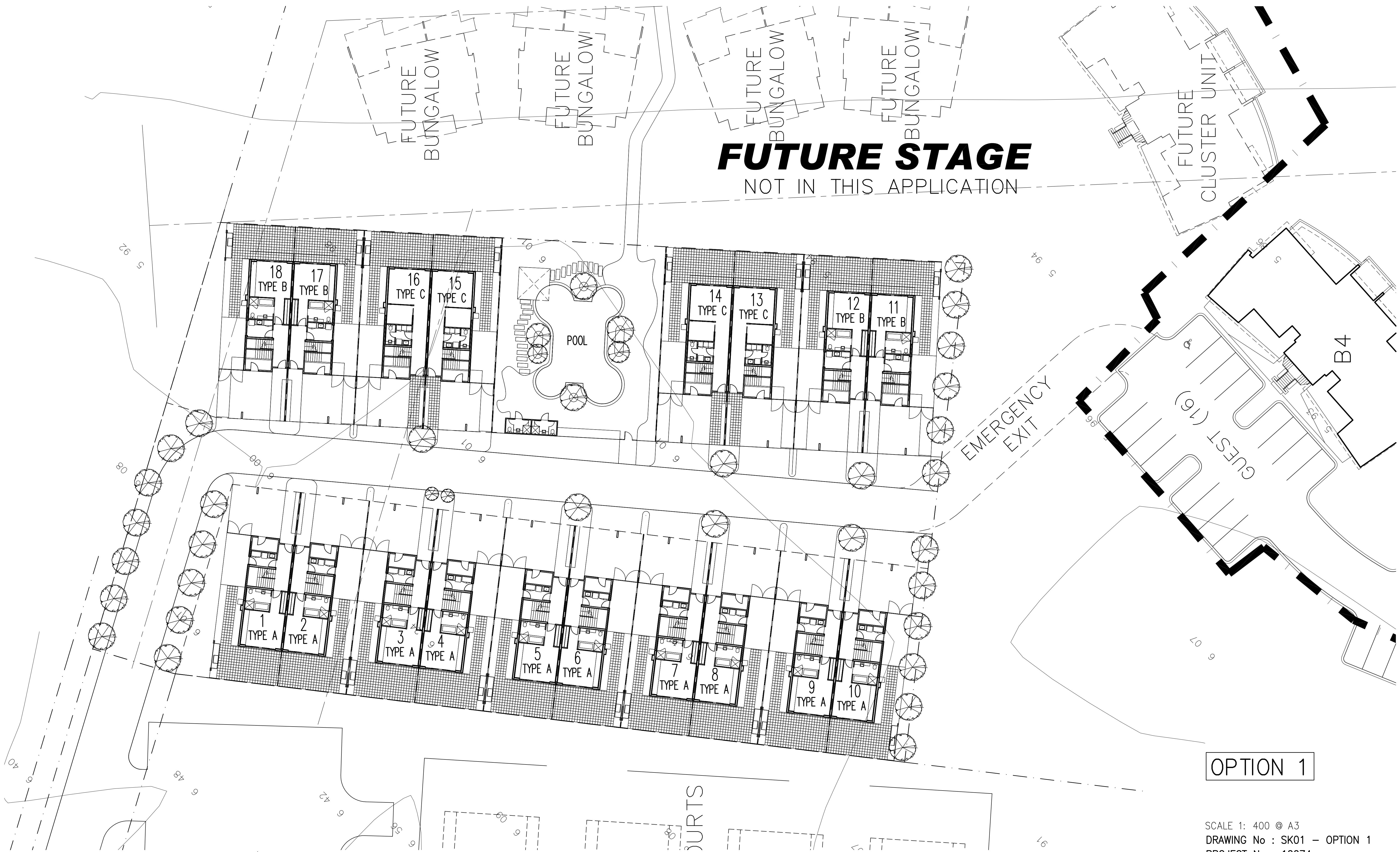
OVERALL GROUND FLOOR PLAN SCALE 1:200 @ A1
