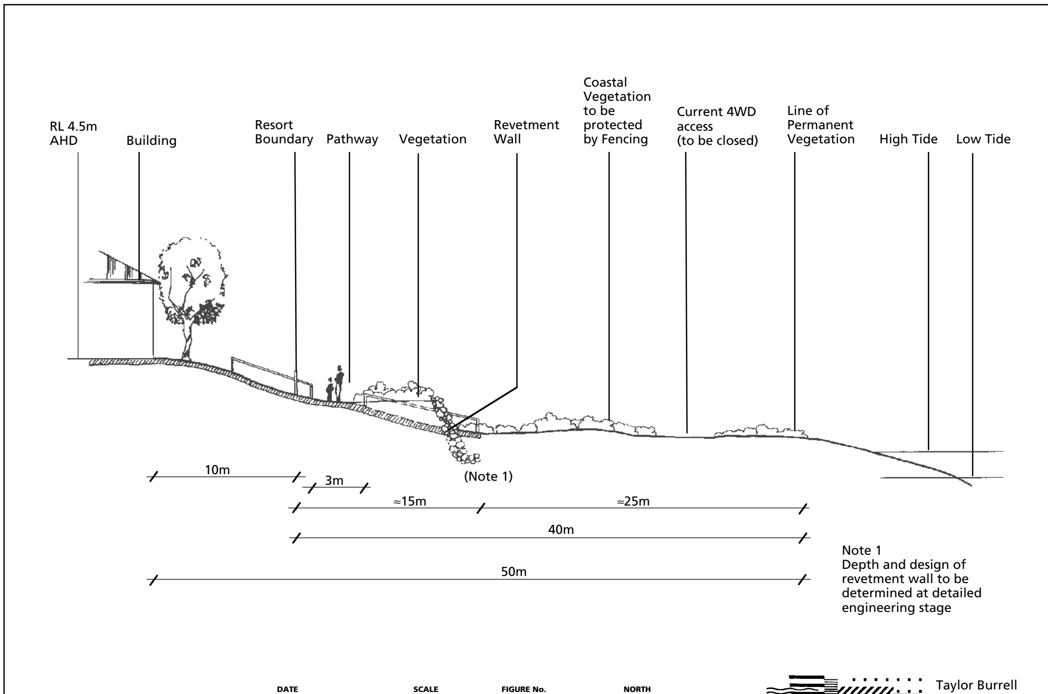
TYPICAL FORESHORE CROSS SECTION BASED ON THE 40m SECTION
