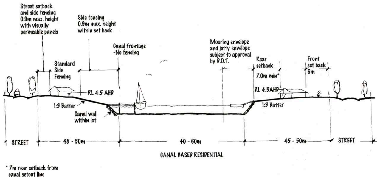
Figure 3: Precinct A Typical Cross-section
