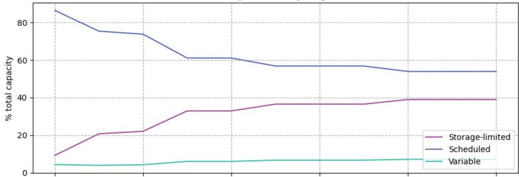
Proportional Capacity
