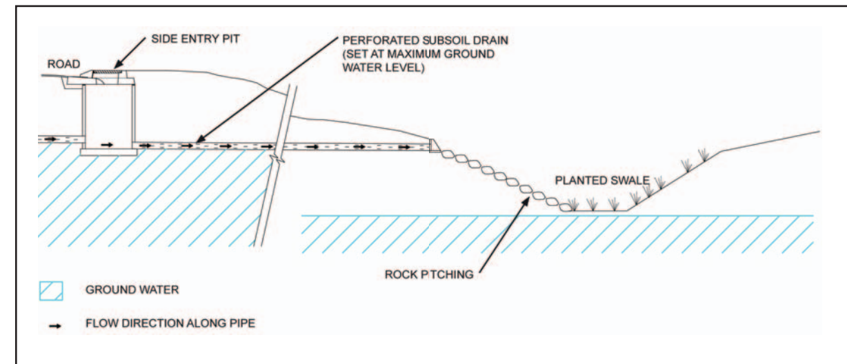
Figure 10 - Indicative design for groundwater level control
