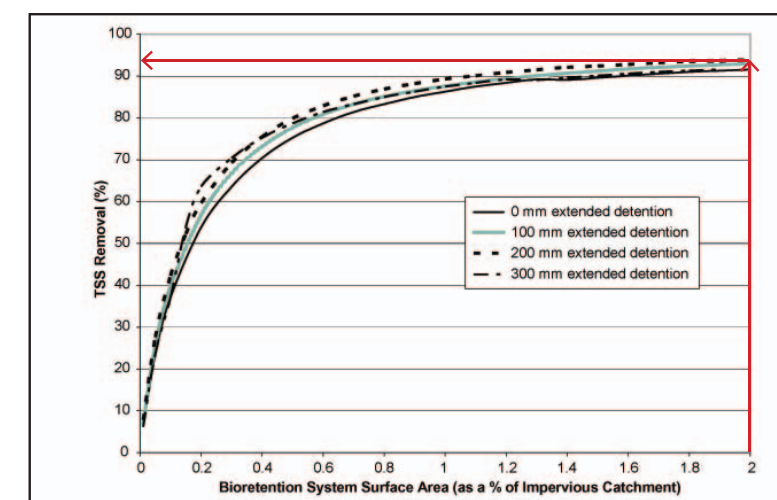
Figure 13 - Bioretention System TSS removal performance
