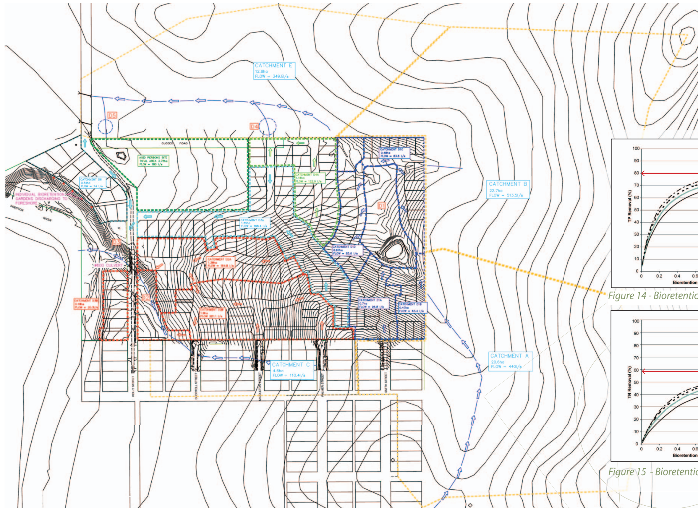
Figure 16 - 1:1 year storm event plan
