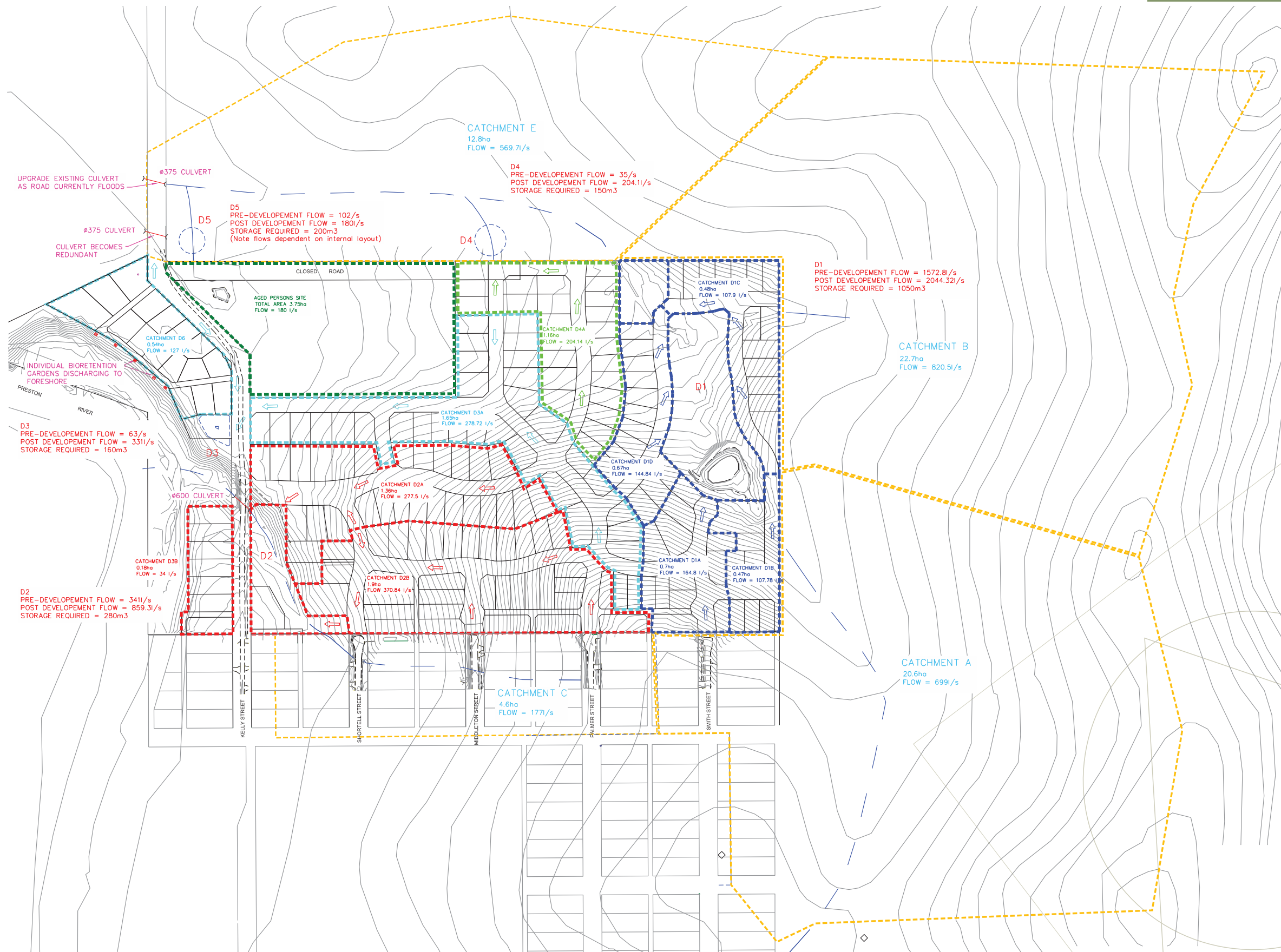
Figure 19 - 1:5 year flood event plan
