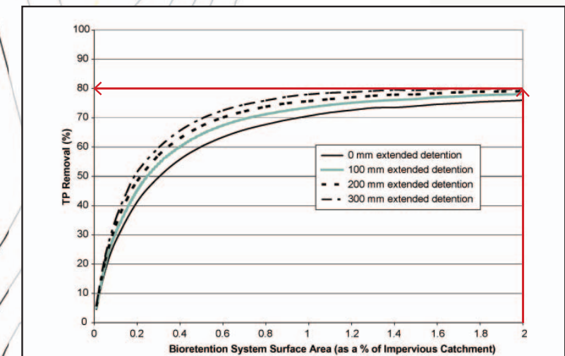
Figure 14 - Bioretention System TP removal performance
