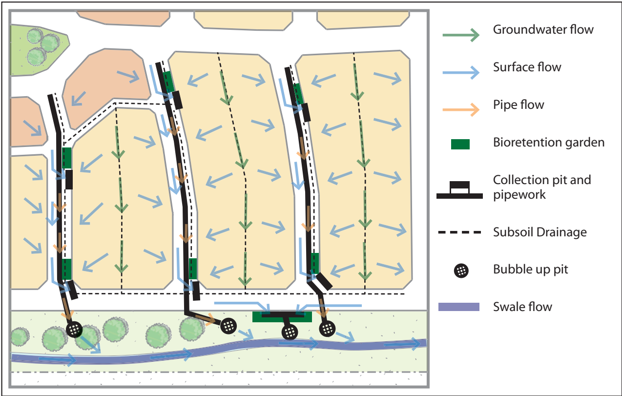
Figure 18 - Enlargement showing 1:5 stormwater
