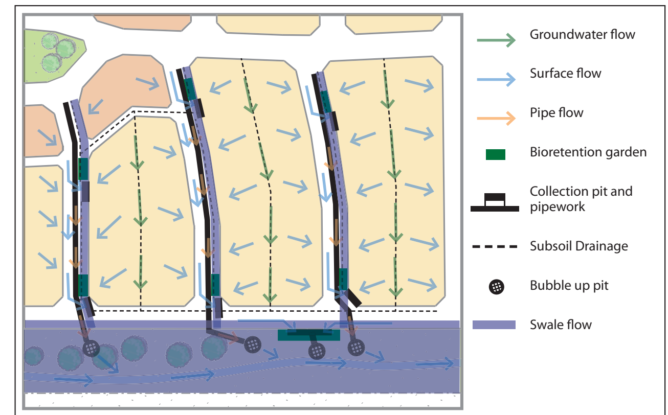
Figure 20- Enlargement showing 1:100 flood flow
