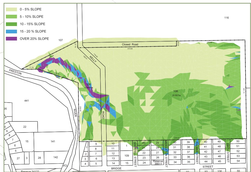
Figure 5 - Slope Analysis Plan
