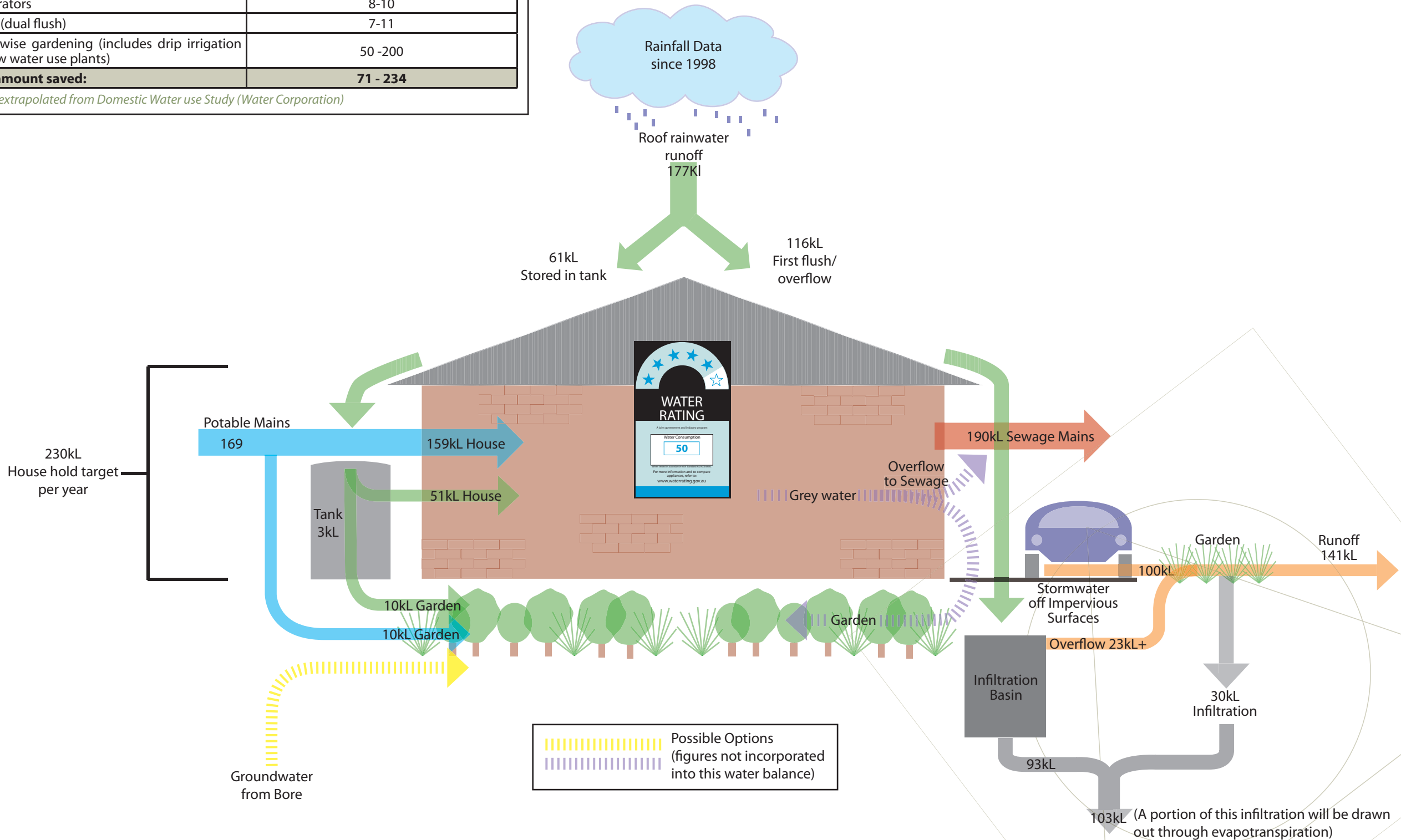
Figure 23 - Water Conservation Strategy
