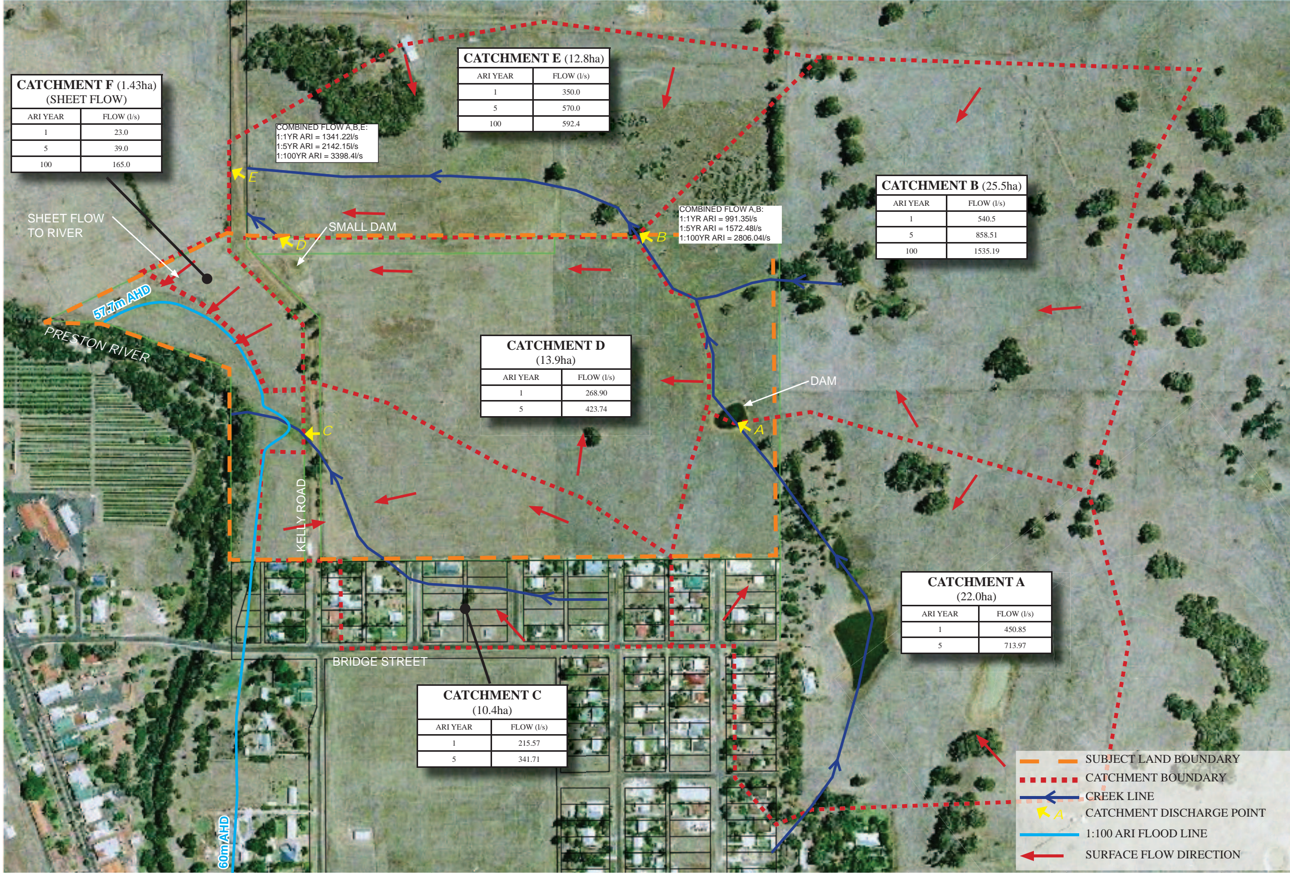
Figure 7 - Existing Drainage and Catchments
