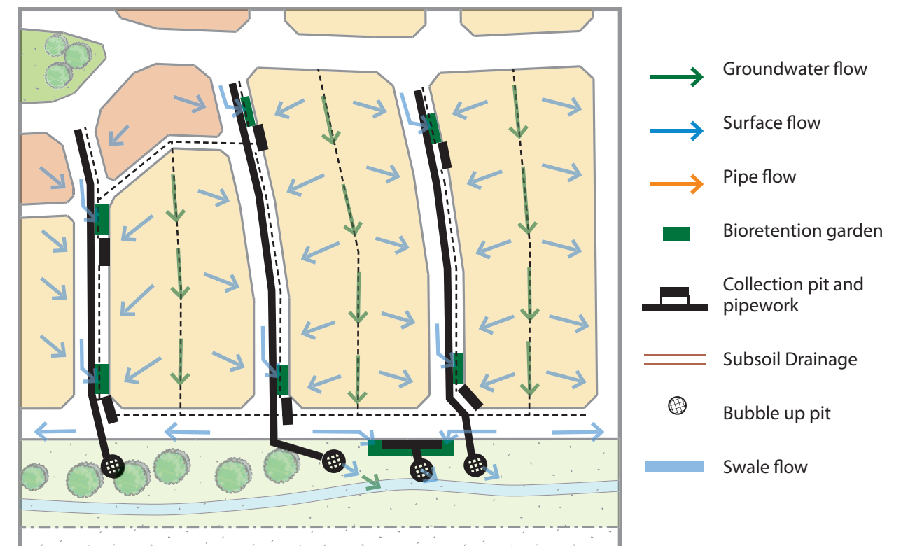
Figure 12 - Enlargement showing 1:1 Stormwater Management
