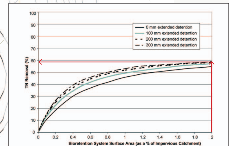
Figure 15 - Bioretention System TN removal performance
