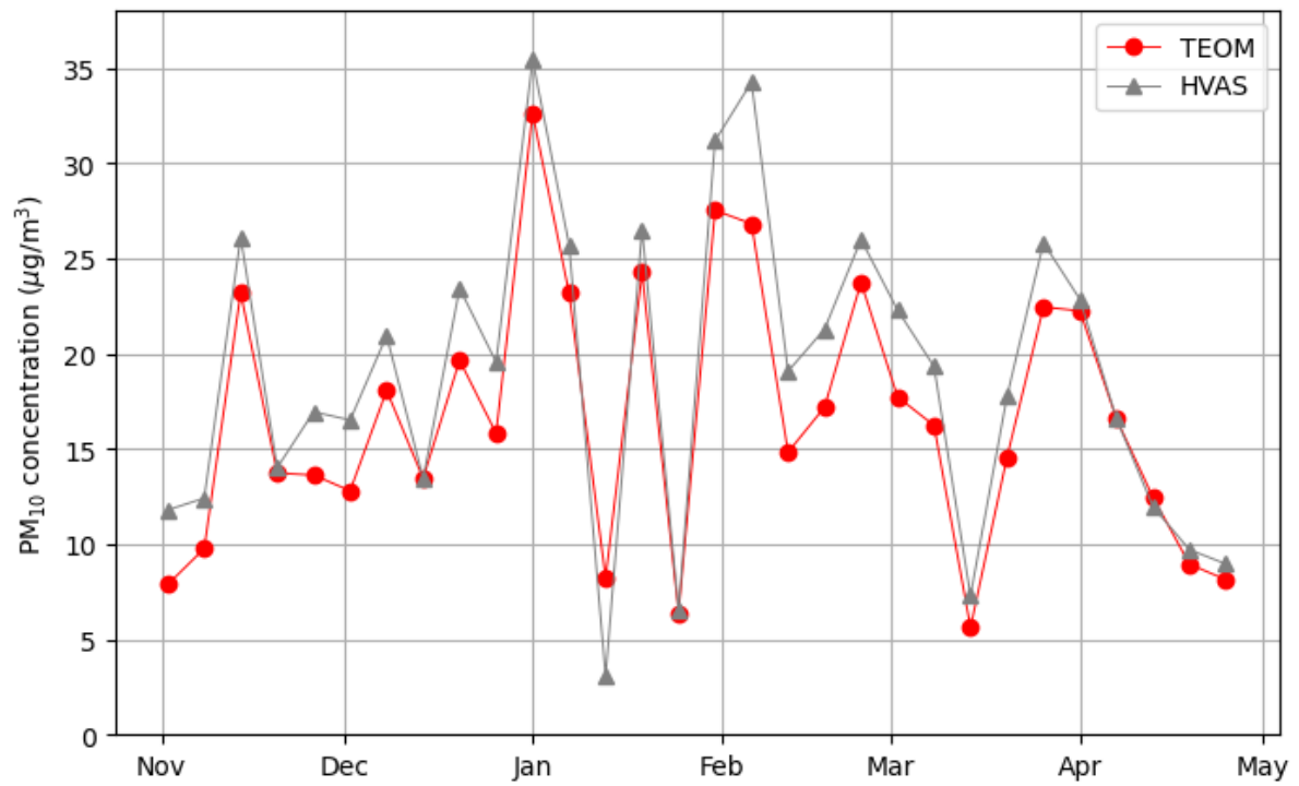
Figure A1-5 HVAS and TEOM daily PM 10 comparison
