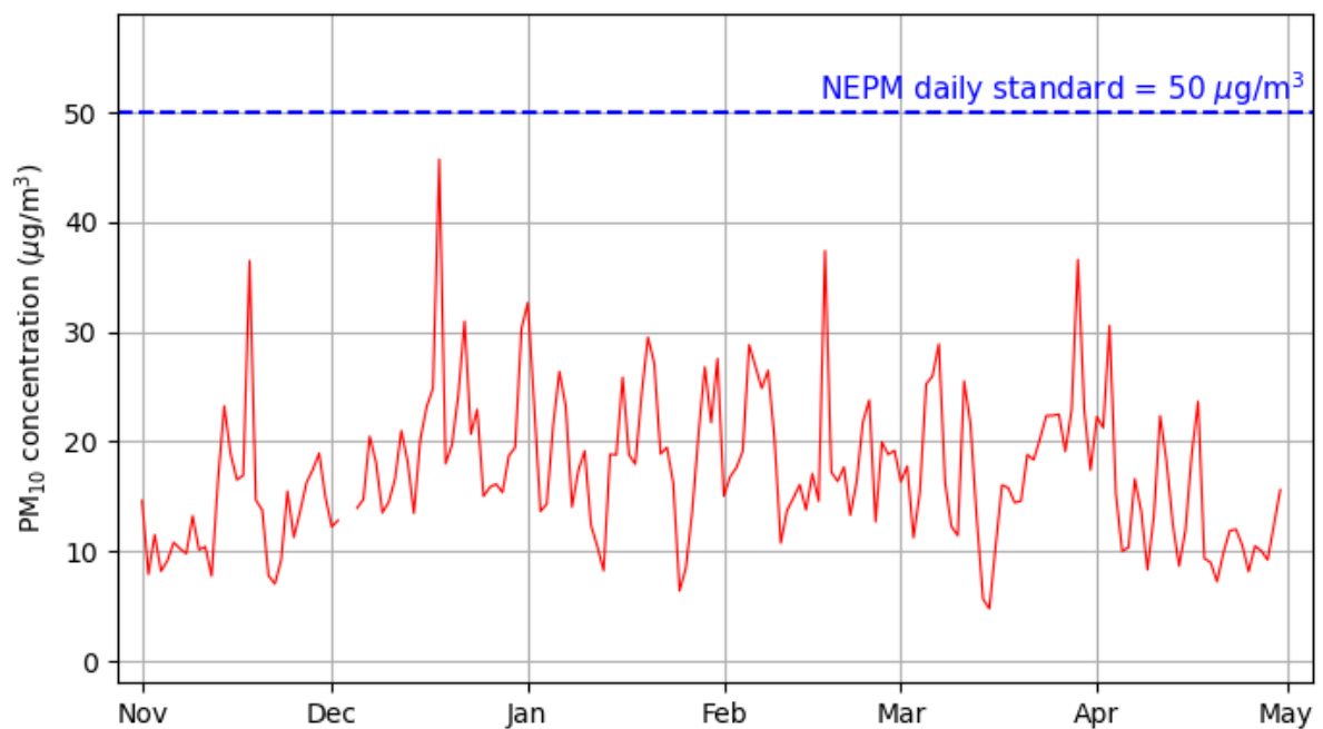
Figure A1-2 TEOM daily PM 10 concentrations and NEPM guideline (50 µg/m³)
