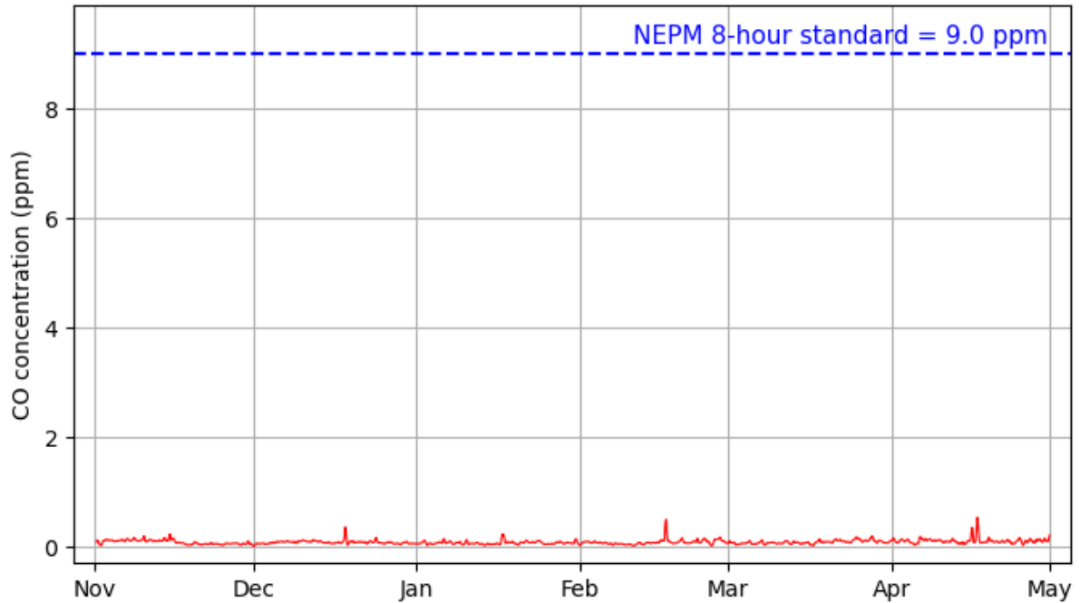
Figure A6-1 8-hourly CO concentrations and NEPM guideline (9.0 ppm)
