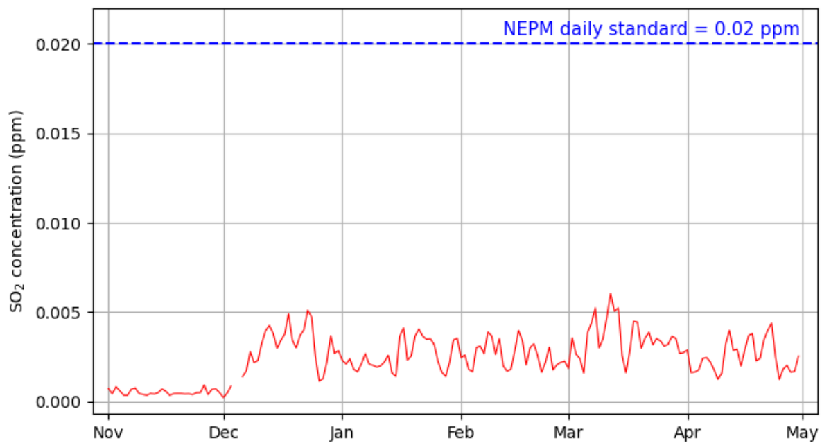
Figure A6-5 Daily SO 2 concentrations and NEPM guideline (0.02 ppm)
