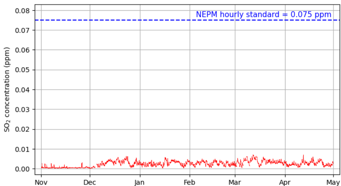
Figure A6-4 Hourly SO_2 concentrations and NEPM guideline (0.075 ppm)
