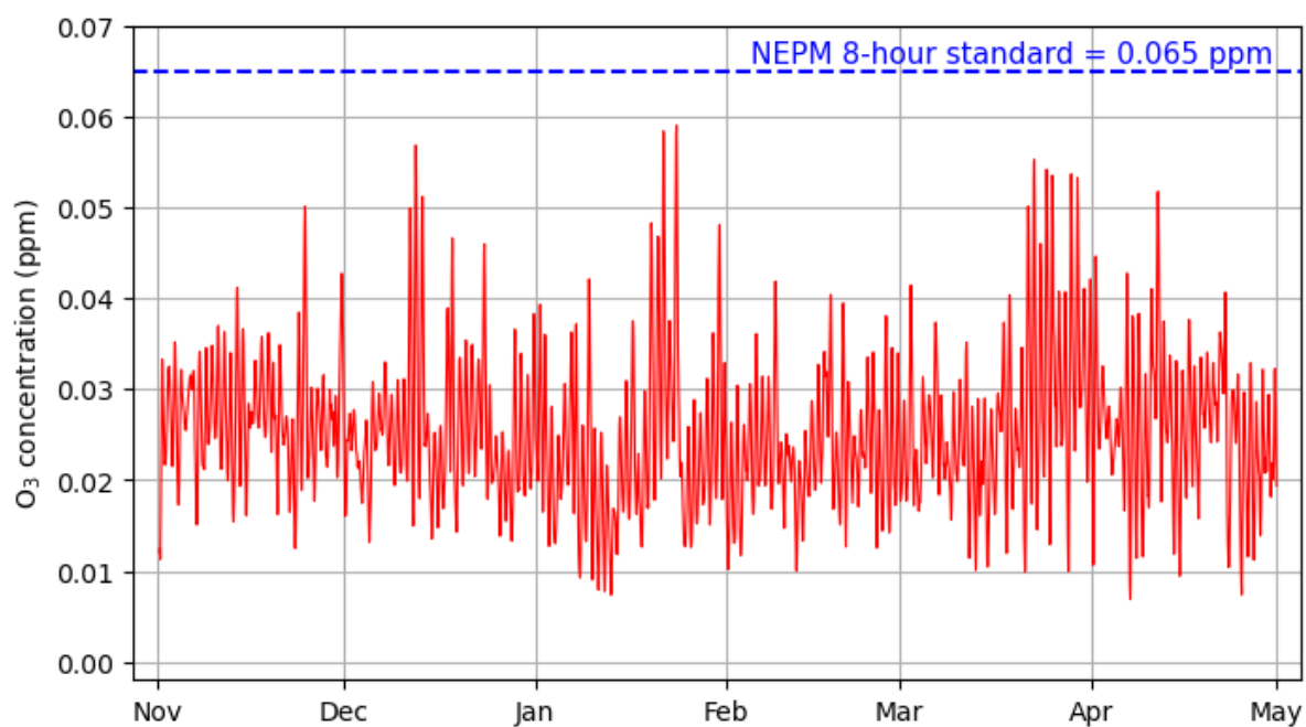
Figure A6-3 8-hourly O_3 concentrations and NEPM guideline (0.065 ppm)
