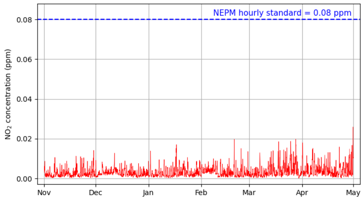
Figure A6-2 Hourly NO 2 concentrations and NEPM guideline (0.08 ppm)
