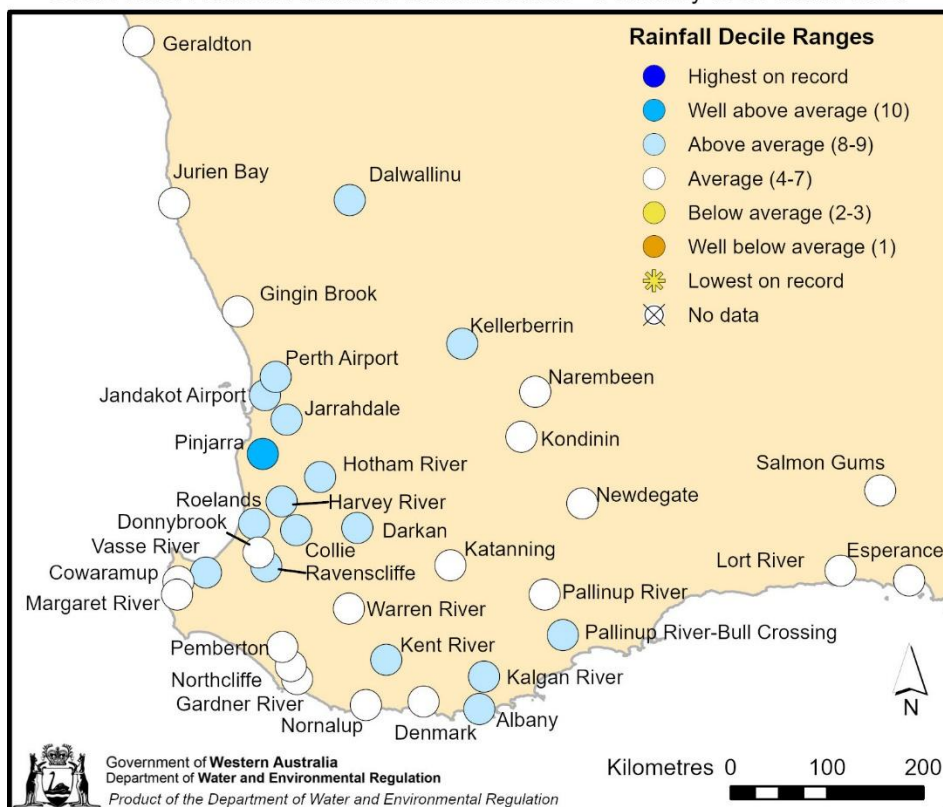
South West Western Australia Rainfall Deciles - 1 January to 31 March 2026
