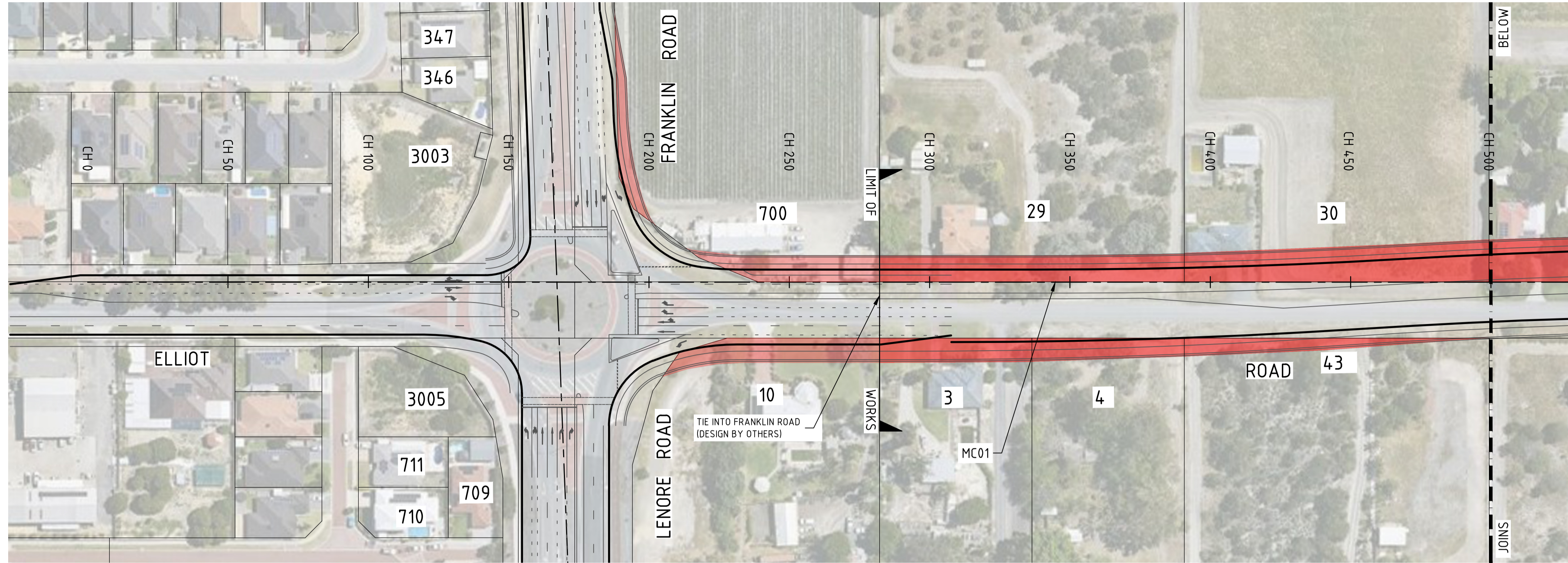
PLAN 1:1000
