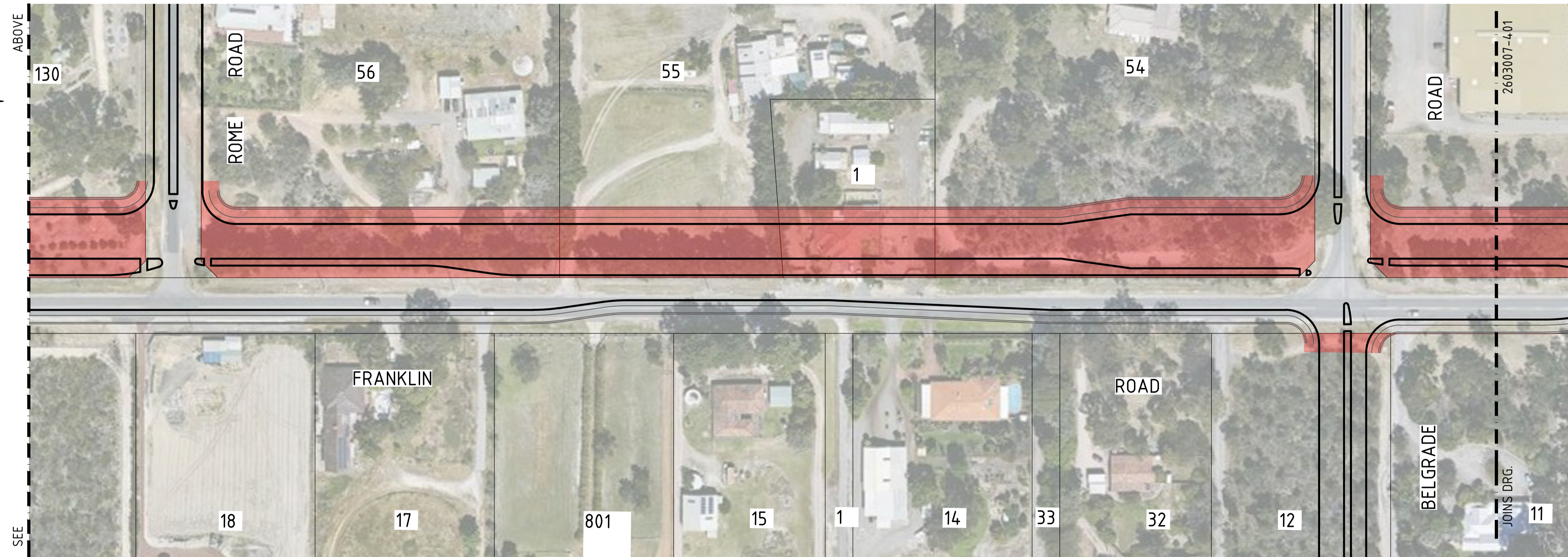
PLAN CONT. 1:1000
