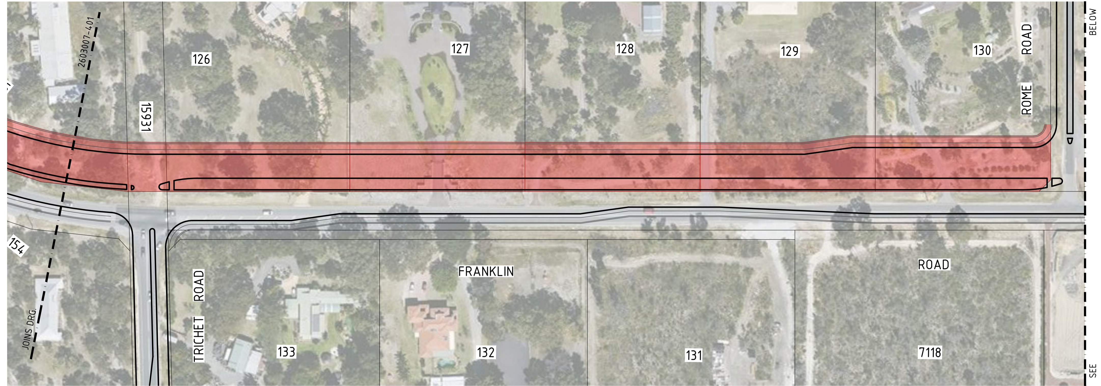
PLAN CONT. 1:1000
