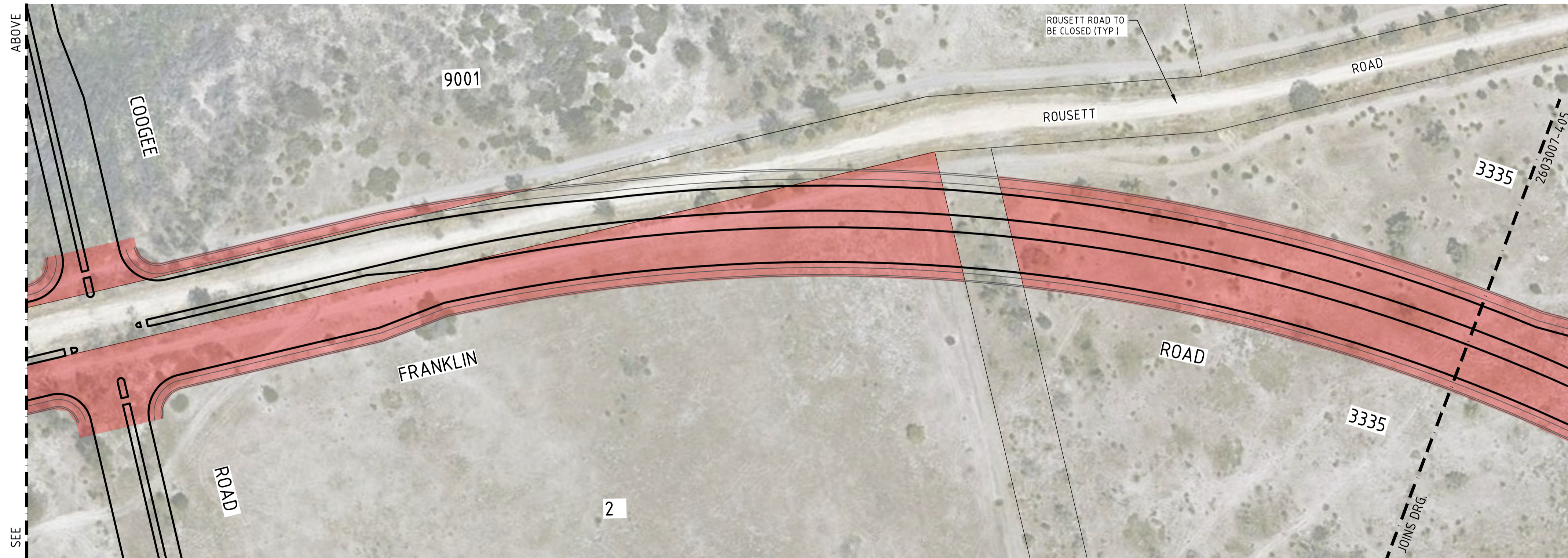
PLAN CONT. 1:1000
