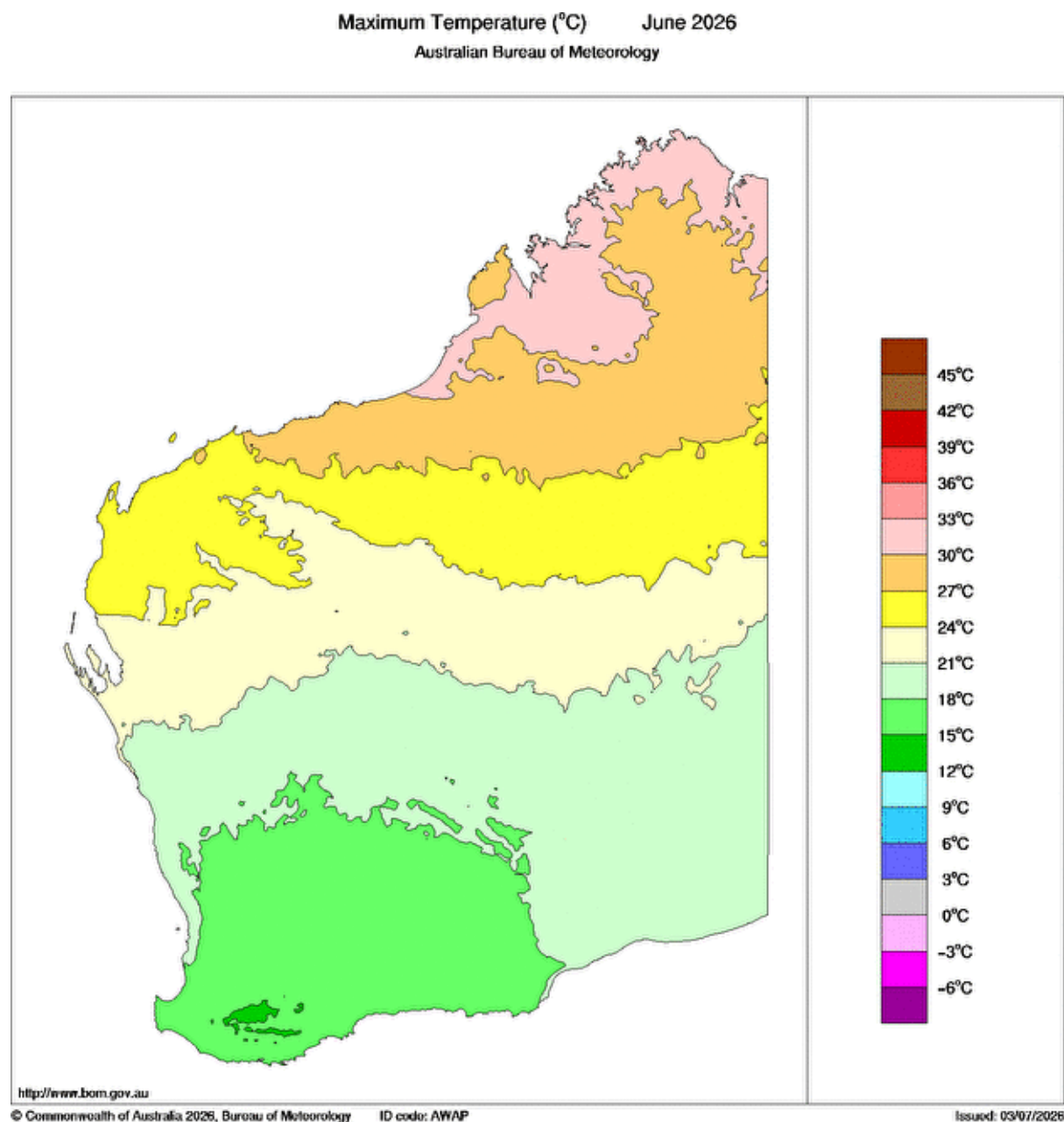
Map 3: Mean maximum temperature (°C) for June 2026
