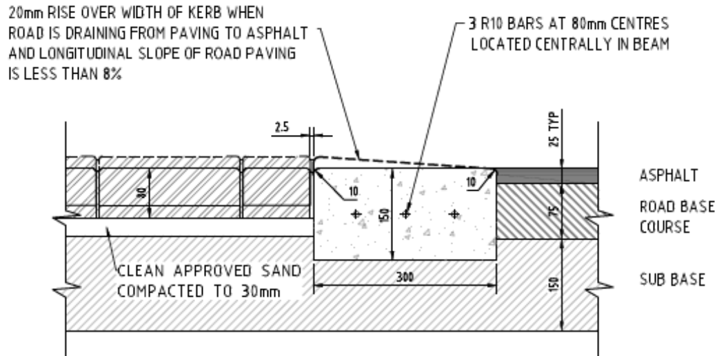
FIGURE 3.2: KERBING PROFILES
