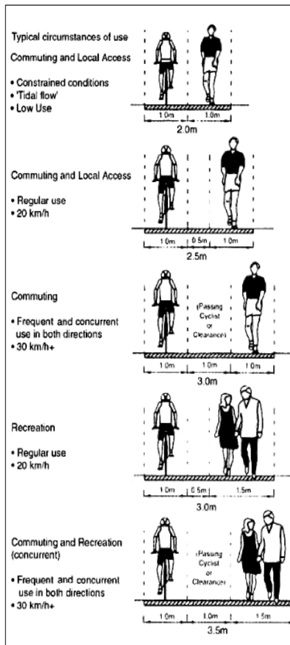
FIGURE 5.2: SHARED PATHS
