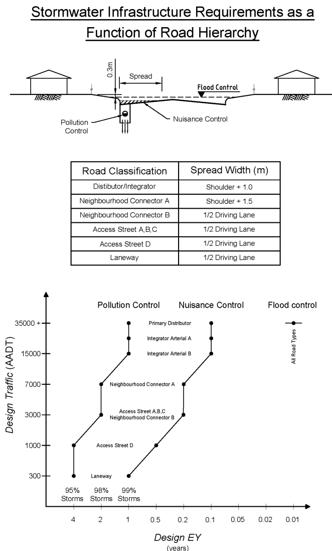
Figure 4.5: Stormwater infrastructure requirements as a function of road hierarchy Source: Evangelisti, Edwards and Barry, 2016
