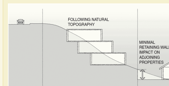
Figure 55: Development on steep or undulating sites should be designed to minimise the amount of cut and fill required. Buildings should have a form that responds to the natural topography of the area.
