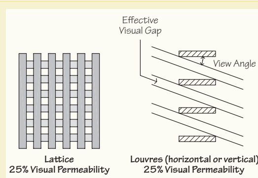
Figure 61: Example of screening by which visual permeability can be limited. Note that a view angle of 45 degrees to the side is the limit of the cone of vision as defined in the R-Codes Volume 1, and no screening is required outside these limits.
