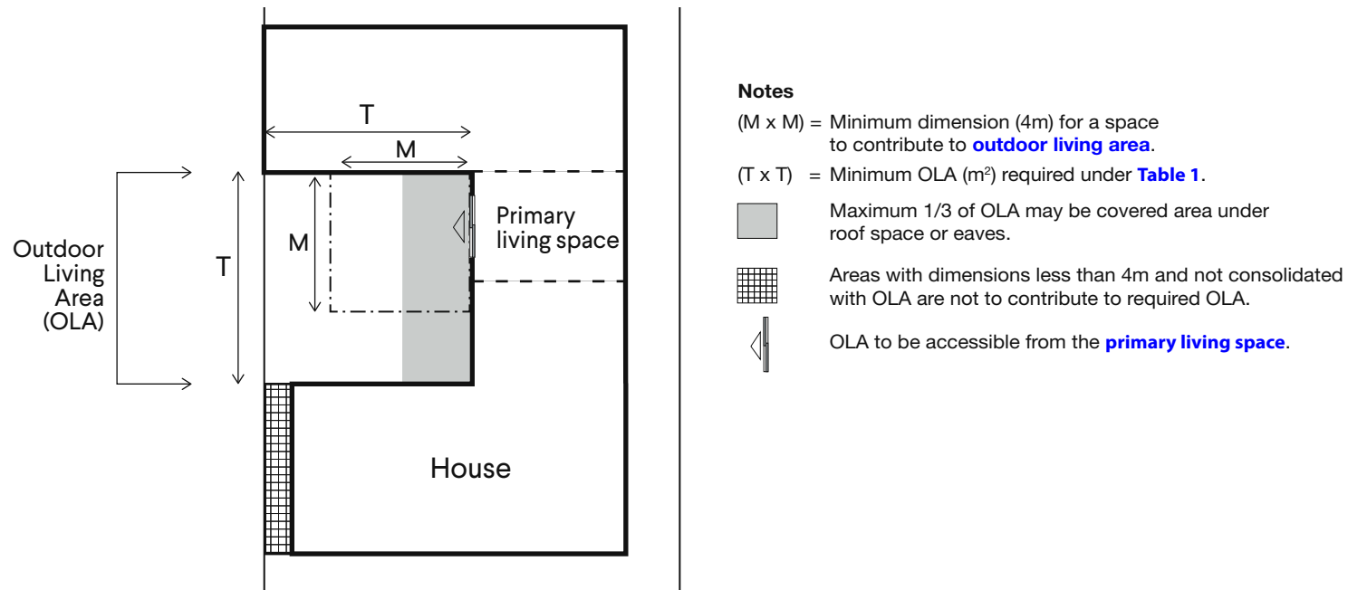
Figure 13 – Dimensions and calculations for outdoor living areas (Clause 5.3.1 C1.1)
