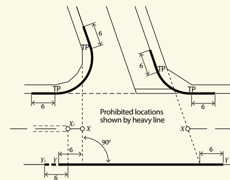
AS2890.1 - Prohibited locations of access driveways
