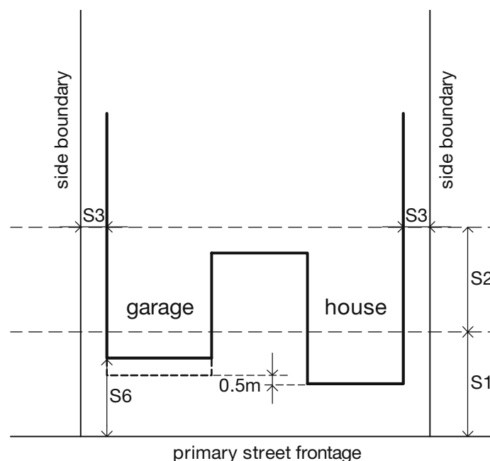
Figure 8b – Garage setbacks (clause 5.2.1 C1.1)
