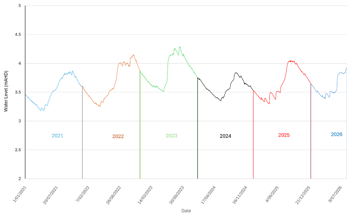
Esperance groundwater tracking - August 2026
