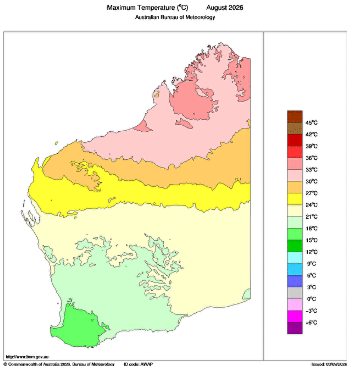
Map 3: Mean maximum temperature (°C) for August 2026
